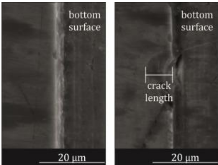
Fig. 9. Edge crack length for C100–C145 and grain size of 1 \mu\text{m} (left) and C100–C145 and grain size of 2 \mu\text{m} (right). (Reprinted from CIRP Annals - Manufacturing Technology, 64/1, Aurich JC, Carrella M, Walk M, Micro grinding with ultra-small micro pencil grinding tools using an integrated machine tool, 325–328, Copyright (2015), with permission from Elsevier).
