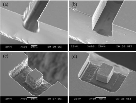
Fig. 8. Micro-structures machined by (a,c) ECDM and (b,d) then ground by a PCD tool. (Reprinted from International Journal of Precision Engineering and Manufacturing, 14/1, Xuan Doan Cao, Bo Hyun Kim, Chong Nam Chu, Hybrid micromachining of glass using ECDM and micro grinding, 5–10, Copyright (2013), with permission from Elsevier).
