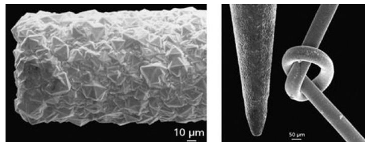
Fig. 7. Micro-CVD diamond-coated grinding tools (Reprinted from International Journal of Machine Tools and Manufacture , 50/4, Jan Gäbler, Sven Pleger, Precision and micro CVD diamond-coated grinding tools, 420–424, Copyright (2010), with permission from Elsevier).
