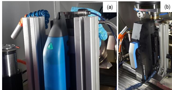
Fig. 18. Measurement setup for the surface roughness a) using the tactile surface roughness tester, b) using the confocal microscope
