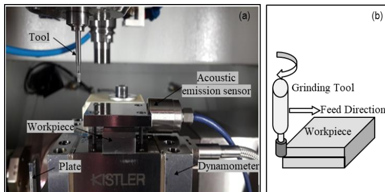
Fig. 17. a) Experimental setup, b) schematic of the grinding process
