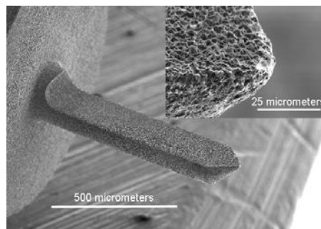
Fig. 12. SEM image of a conical tipped PCD tool. (Republished with permission of IOPscience, from Micro machining glass with polycrystalline diamond tools shaped by micro electro discharge machining, Morgan CJ, Vallance RR, Marsh ER, 14, 12 and 2004).
