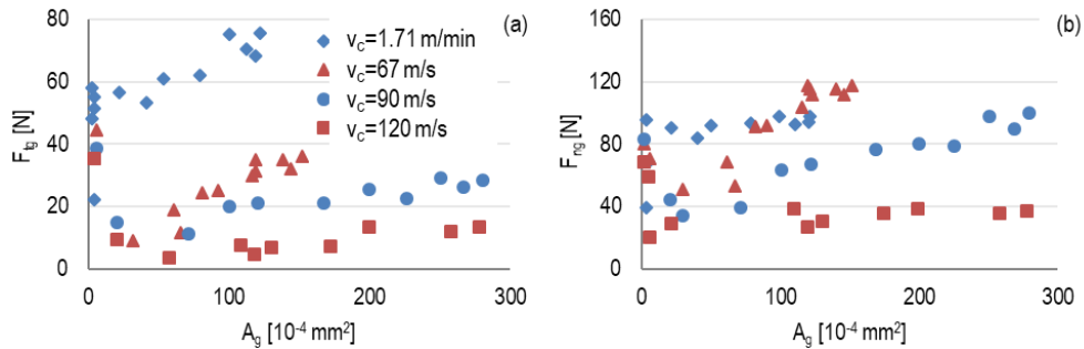
Fig. 14. Single-grit grinding forces: a) normal grinding force, b) tangential grinding force [47]
