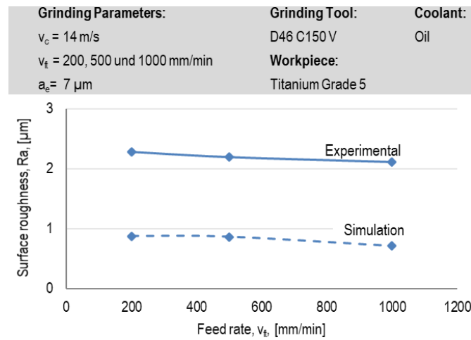
Fig. 27. Surface roughness versus feed rate, v_f
