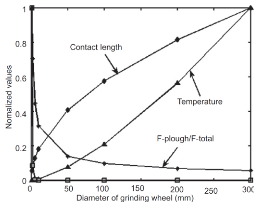
Fig. 13. Variation trend of main parameters according to varying wheel dimensions (Reprinted from International Journal of Machine Tools and Manufacture, 48/15, Hyung Wook Park, Steven Y. Liang, Force modeling of micro-grinding incorporating crystallographic effects, 1658–1667, Copyright (2008), with permission from Elsevier).
