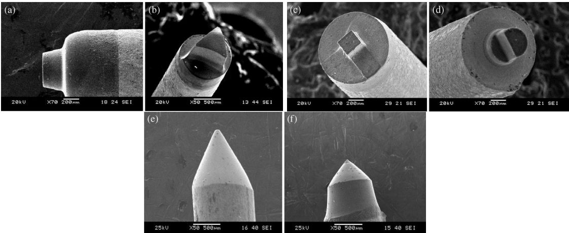
Fig. 11. a) Circular tool, b) triangular tool, c) square tool, d) D-shaped tool, e) conical tool of 60°, and f) conical tool of 90°. (Reprinted by permission from Springer: Springer Nature, The International Journal of Advanced Manufacturing Technology, [32], Fabrication of different geometry cutting tools and their effect on the vertical micro-grinding of BK7 glass, Asma Perveen, Wong Yoke San, Mustafizur Rahman, Copyright (2013)).
