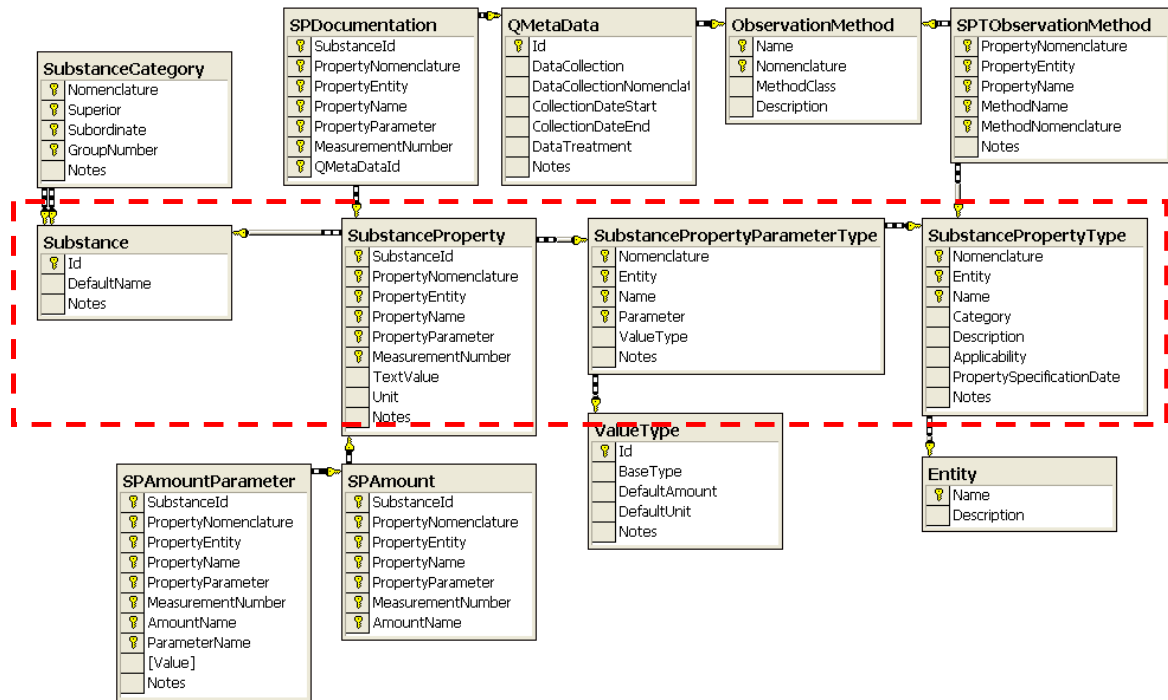
Figure A3.2 An extraction of the IMPRESS reference data model for structured storage of substance property data.
