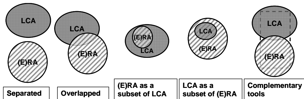
Figure 4 Alternative approaches of combining LCA and (E)RA in terms of simplified Venn diagrams.
