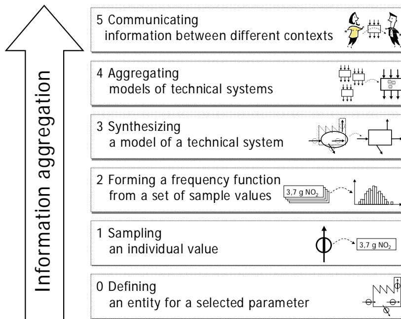
Figure 3 The information aggregation phases in the PHASETS model.
