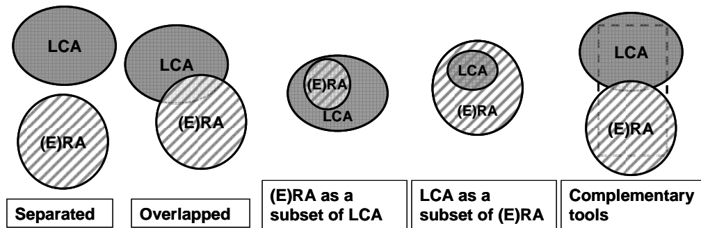
Figure A2.1 Alternative approaches of combining LCA and (E)RA in terms of simplified Venn diagrams.
