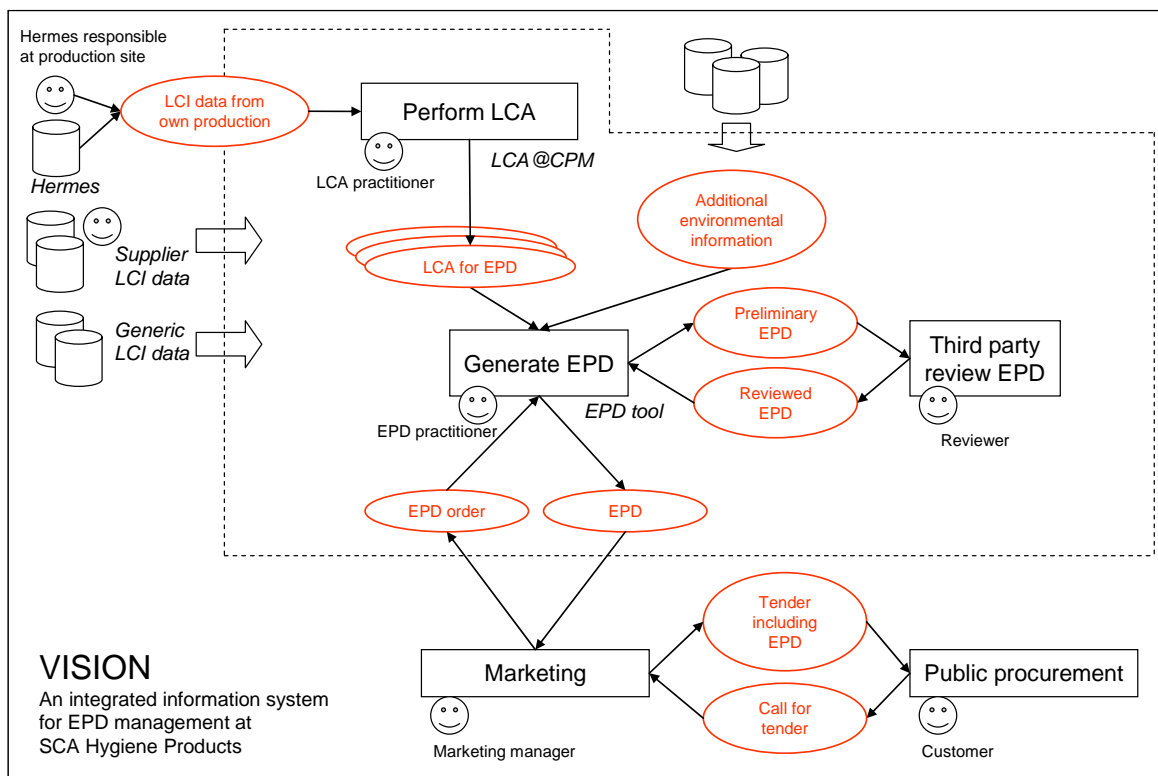
Figure 2 presents the vision of the integrated information system for EPD management at SCA Hygiene Products.
