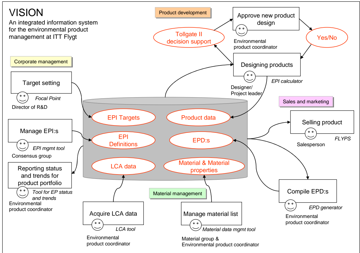
Figure 3 presents the vision of an integrated information system for the environmental product management at ITT Flygt.
