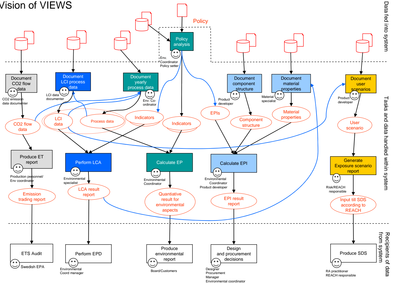
Figure 1 The vision of the integrated information system VIEWS.
