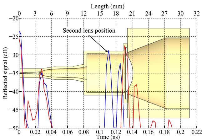
FIG. 9. Time-domain measurements of the spline horn and Topas lens. Two measurements (corresponding to the blue and red lines) were made, where the distance between the horn aperture and the lens was varied. NB: The length scale at the top is with reference to the physical size of the horn/lens plotted in the figure. The second roundtrip after reflections is thus neglected in this scale that differs by a factor of two compared to the time scale at the bottom.
