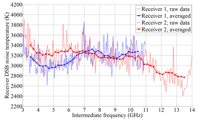
FIG. 12. Receiver DSB noise temperature as a function of intermediate frequency for the 874 GHz flight receivers for ISMAR. The data are corrected for losses in the setup. An averaging window of width 1 GHz was used. The temperature of the front-ends was regulated to 40 °C.
