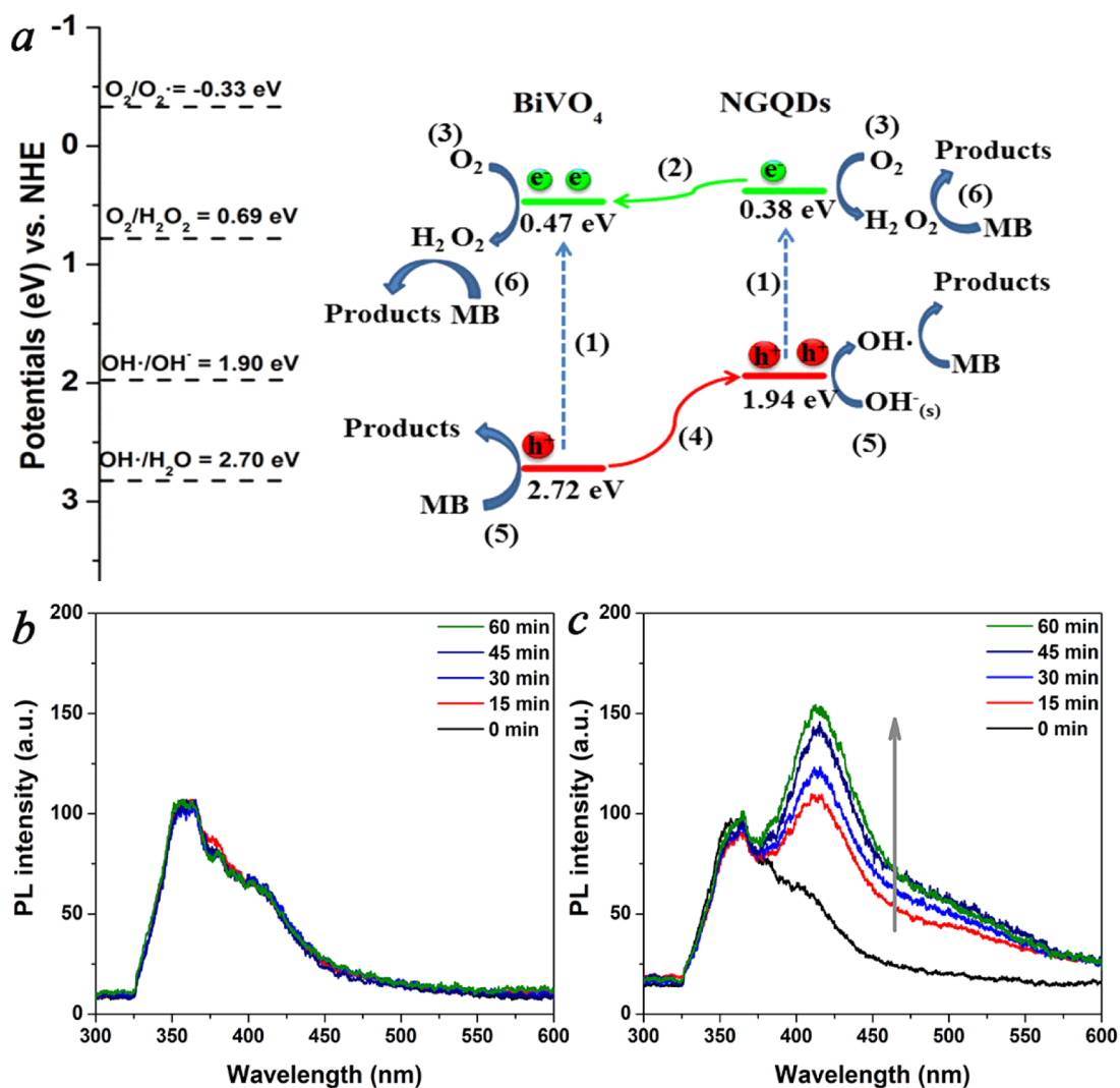
Figure 5. (a) Schematic illustration of the proposed photocatalytic mechanism and interfacial charge transport for the NGQDs/ \text{BiVO}_4 nanojunction composite under visible-light irradiation ( \lambda > 420 nm). \cdot\text{OH} trapping PL spectra of (b) the pristine \text{BiVO}_4 and (c) 5 wt % NGQDs/ \text{BiVO}_4 samples by TA hydroxylation. The observed PL peak at about 360 nm originated from the sampling capillary glass tube. 43
