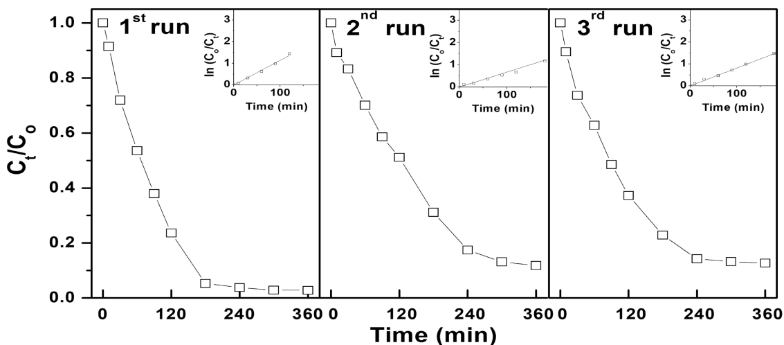
Figure 6. Recyclability of the 5 wt % NGQDs/ \text{BiVO}_4 nanocomposite for photodegradation of MB. Insets: the corresponding first-order kinetic fitting curves.
