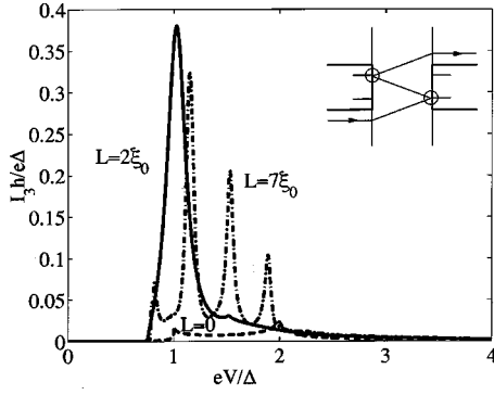
FIG. 10. Three-particle current in symmetric junctions L_l=L_r=L/2 for different lengths; the junction transparency is D=0.1 . The MAR path with two overlapping resonances, shown in the inset, generates a current peak with height proportional to D .
