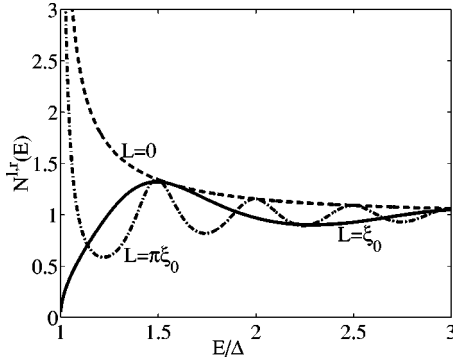
FIG. 5. Density of states in the N region for different lengths L of the region. Singular behavior of the DOS for short junctions, L = 0 (equal to the DOS in a superconductor), is suppressed for finite-length junctions. The amplitude of the first oscillation increases as the length increases, indicating accumulation of the spectral weight at the energy-gap edge and formation of a bound state for L = \pi\xi_0 .
