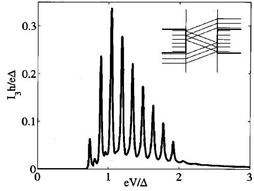
FIG. 11. “Peak triangle” of three-particle current for long junction: L_l=L_r=L=10\xi_0 , D=0.1 . Every peak of the triangle consists of a number of tightly positioned resonances due to nearly equidistant bound-state spectrum (resonance cluster). The number of resonances in a cluster is, from left to right, 1, 4, 7, 6, 5, 4, 3, 2, 1. The inset shows an example of resonant MAR paths forming a cluster.
