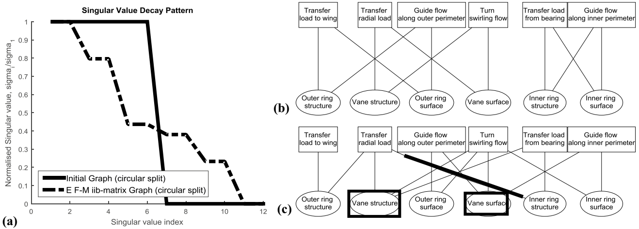
Fig. 25 a SVD decay pattern for the circular split vane in Fig. 21d. b Initial graph; every section has the same degree centrality and each cross-edge has the same betweenness centrality and thus, section and
