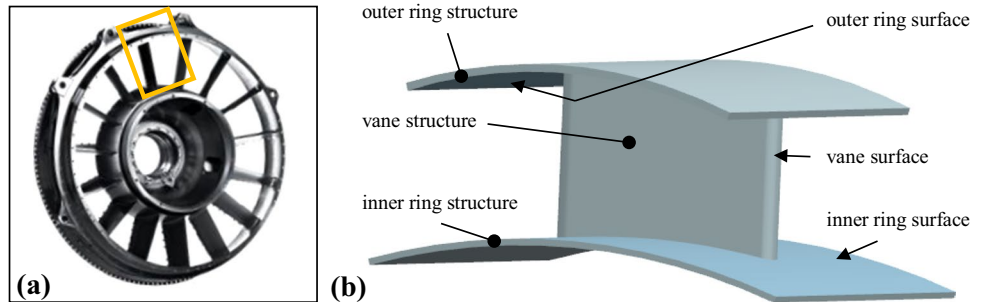
Fig. 20 a A turbine rear structures with a vane section highlighted. b A simplified view of the vane with different sections
