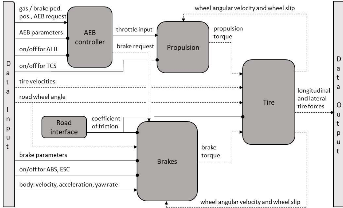
Figure 8: Structure of the brakes, propulsion, and tires model. Parameter-flow (time-independent) is marked with \text{---}\bullet and variable-flow (time-dependent) with \text{---}\rightarrow . Vectorized connection statements are shown with a dashed line.
