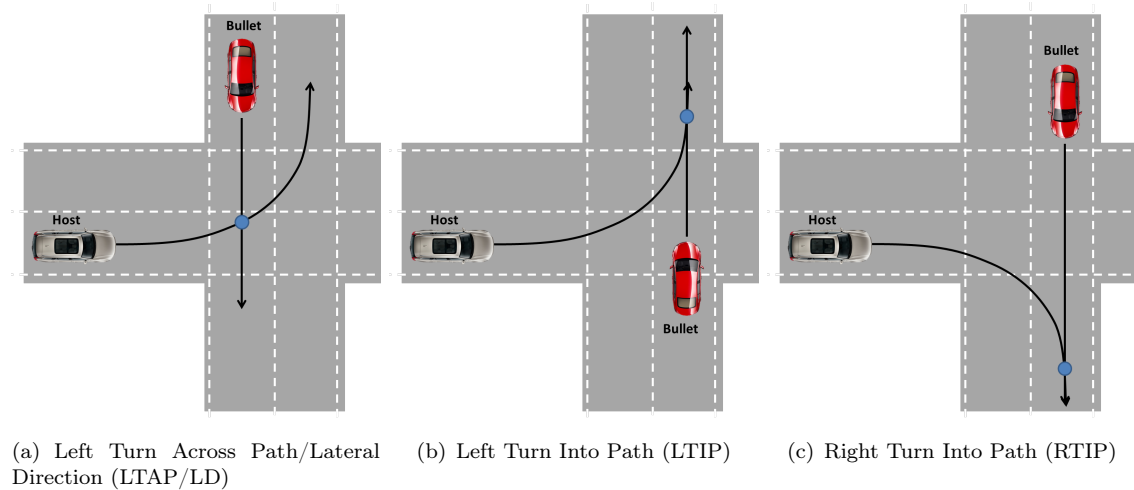
Figure 14 Intersection accidents
