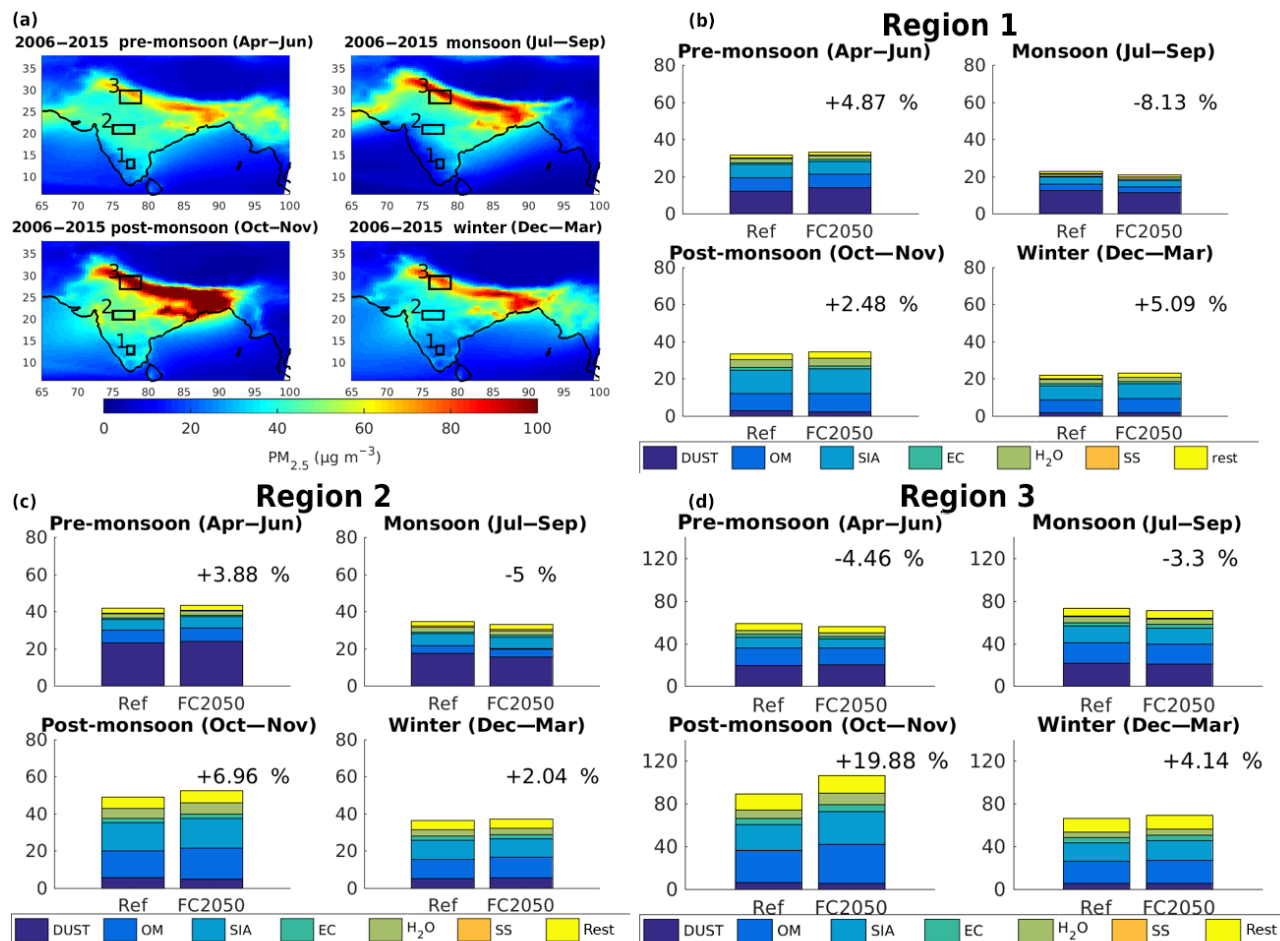
Figure 10. Seasonal distribution of surface \text{PM}_{2.5} concentrations (in \mu\text{g m}^{-3} ) for the reference scenario, and seasonal composition of \text{PM}_{2.5} (in \mu\text{g m}^{-3} ) for the three regions highlighted by black boxes on the map for the reference and the FC2050 scenarios. The black percent corresponds to the relative difference in \text{PM}_{2.5} between both scenarios for each region. Note the different y axis for Region 3.
