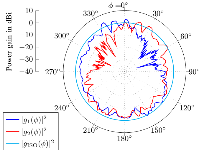
Figure 4.1: Measured directive gains of two monopole antennas placed on the roof of a Volvo XC90 in the azimuth plane. The front of the car coincides with \phi = 0 .
