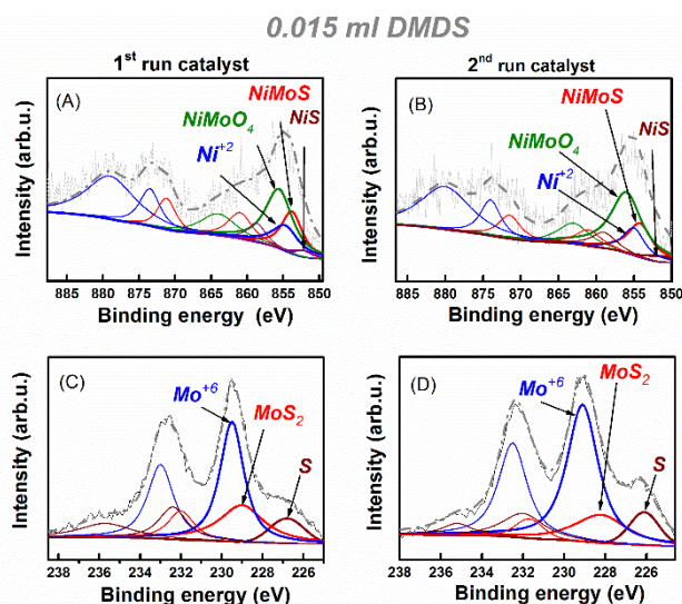
Figure 24. XPS deconvolution of the Ni 2p, Mo 3d and S 2s for: (A) Ni of first run catalyst (B) Ni of second run catalysts (C) Mo of first run catalyst (D) Mo of second run catalysts. Catalysts were maintained with 0.015 mL DMDS.
