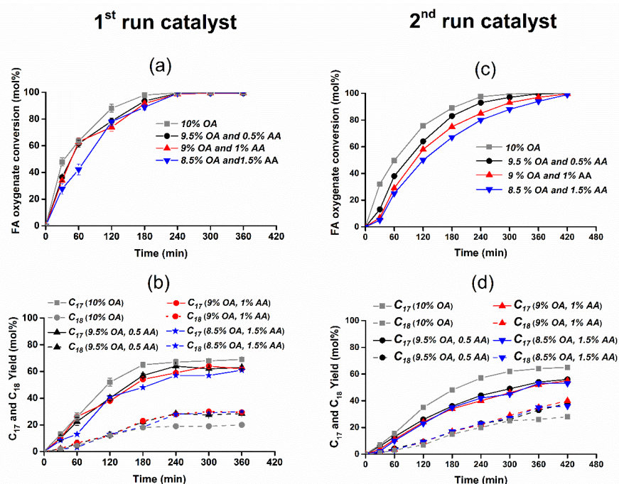
Figure 29. Effect of the abietic acid (AA) concentration on: (a) fatty acid (FA) oxygenate conversion rate of oleic acid (OA) portion of feed with 1 st run catalysts, (b) yields of heptadecane (C 17 ) and octadecane (C 18 ) with 1 st run catalysts, (c) fatty acid (FA) oxygenate conversion rate of oleic acid (OA) portion of feed with 2 nd run catalysts, (d) yields of heptadecane (C 17 ) and octadecane (C 18 ) with 2 nd run catalysts. Experiments were performed at 320 °C, with 500 mg freshly sulfided catalysts, maintained by DMDS (0.1 mL) under pressures 54 -56 bar H 2 .
