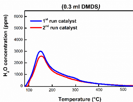
Figure 26. Concentration profile of the H 2 O during the TPO of the first run and second runs catalysts maintained with 0.3 mL DMDS, in 21% O 2 /Ar.
