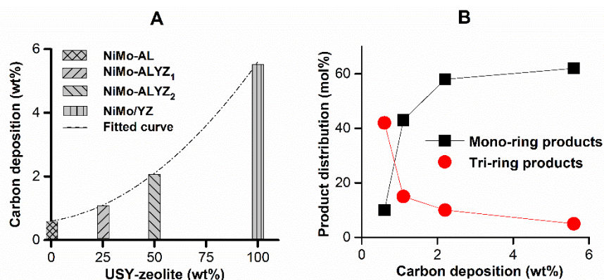
Figure 40. Carbon content versus the USY-zeolite contents (A) and Variation of the mono and tri-ring products versus the carbon deposition of the NiMo catalysts (B). NiMo catalysts supported on USY-zeolite only (NM-YZ), 50 wt% alumina and 50 wt% USY-zeolite (NM-ALYZ 2 ), 75 wt% alumina and 25 wt% USY-zeolite (NM-ALYZ 1 ) and alumina only (NM-AL).
