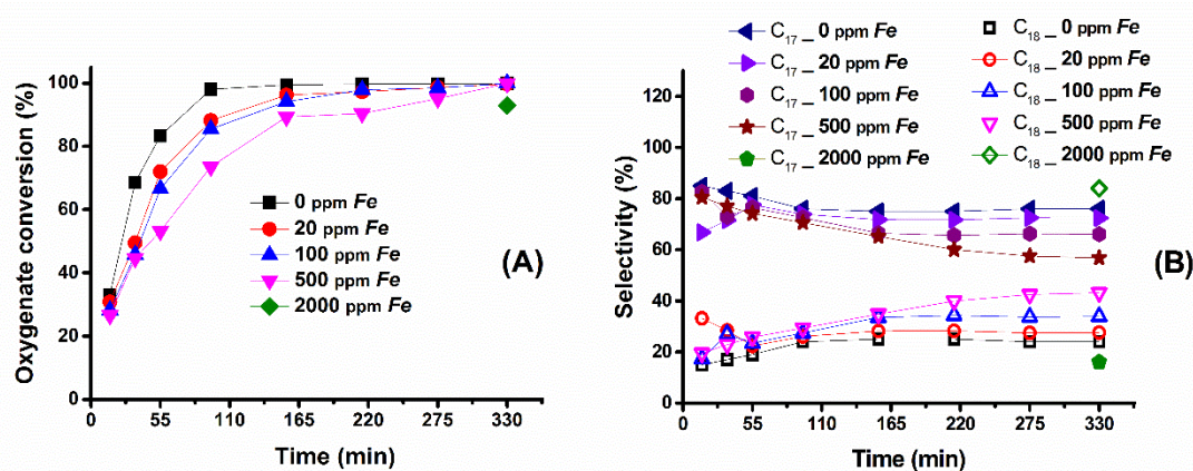
Figure 33. Effect of poison concentration (Fe) on: (A) oxygenate conversion and (B) selectivity for C 17 (heptadecane) and C 18 (octadecane) during HDO of oleic acid over sulfided NiMo/Al 2 O 3 catalyst.
