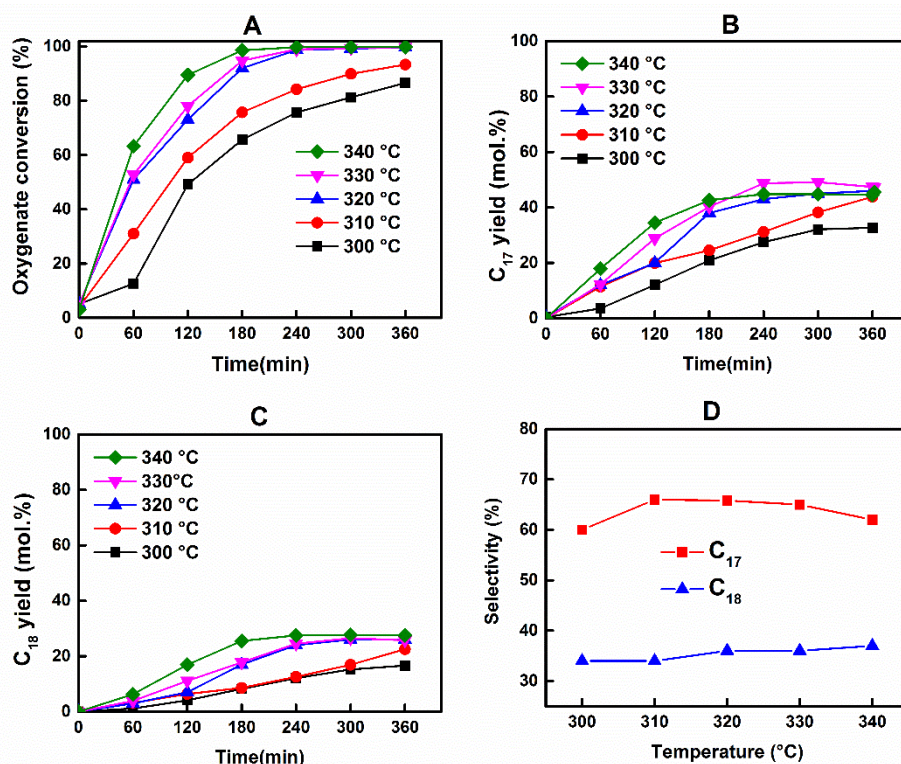
Figure 19. Effect of temperature on: (A) oxygenate conversion (B) yields of heptadecane (C 17 ), (C) yields of octadecane (C 18 ) and (D) selectivity.
