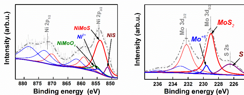
Figure 16. XPS spectra of the Ni 2p, Mo 3d and S 2s core level spectrum for a freshly sulfided sample.
