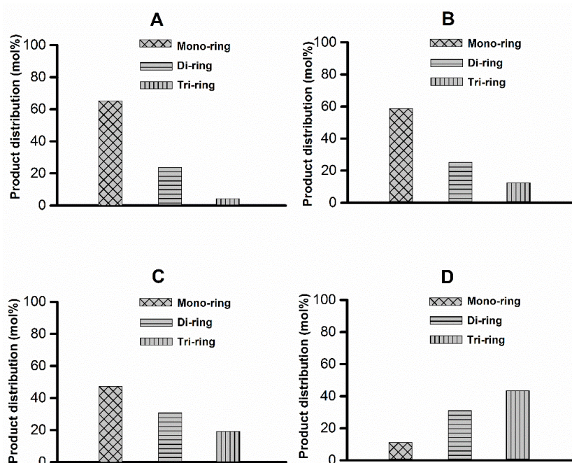
Figure 37. Change of product selectivity over NiMo sulfided catalysts with varying support compositions. Sulfided NiMo catalyst supported on USY-zeolite only (A), 50 wt% alumina and 50 wt% USY-zeolite (B), 75 wt% alumina and 25 wt% USY-zeolite (C) and on alumina only (D).
