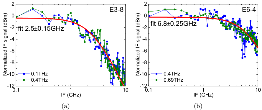
Fig. 6.8: GBW of HEBs (a) E3-8 (20 nm thick, T_c = 38.5 K) at 0.1 THz and 0.4 THz LOs and (b) E6-4 (12 nm thick, T_c = 33.5 K) at 0.4 THz and 0.69 THz.
