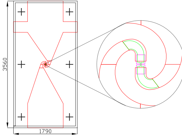
Fig. 4.1: The design of MgB_2 HEB mixer including alignment marks. The dimensions are given in microns.
