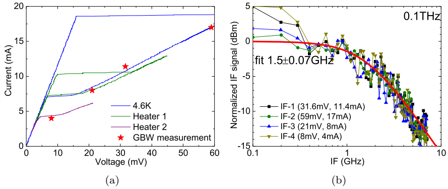
Fig. 6.7: GBW of HEB E2-2 (30 nm thick, T_c = 39.5 K). (a) I-V curves measured in LHe cryostat at various bath temperatures and (b) mixing signal at 0.1 THz at various bias points. (Data adopted from [Paper E])
