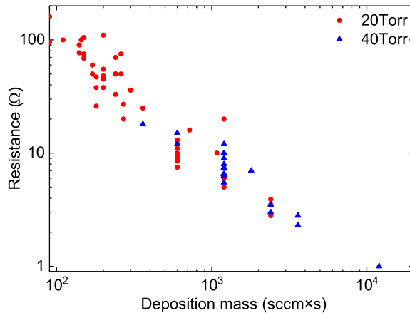
Fig. 3.5: MgB 2 film resistance measured on 5×5 mm 2 size test wafers (SiC) versus deposition mass. Films are deposited at either 20 Torr or 40 Torr.
