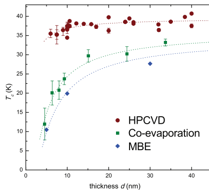
Fig. 3.2: Comparison of different MgB_2 thin film deposition techniques: MBE [174], co-evaporation [175], and HPCVD [172, 176, 177]. Illustration from Ref. [177].
