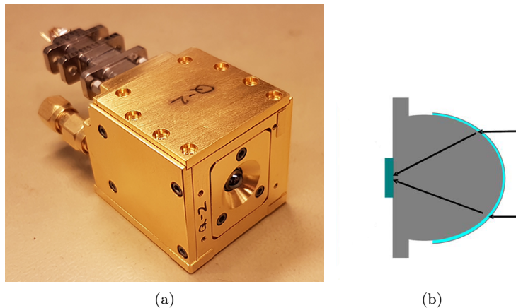
Fig. 2.10: (a) Quasi-optical mixer block used for HIFI instrument of The Hershel Space Observatory. (b) Elliptical dielectric lens with a planar antenna integrated HEB mixer attached. Illustration from [98].
