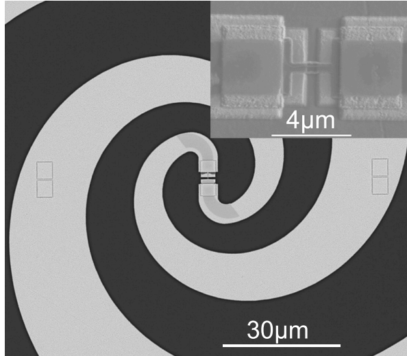
Fig. 4.3: SEM images of MgB_2 HEB made using e-beam lithography based fabrication process.
