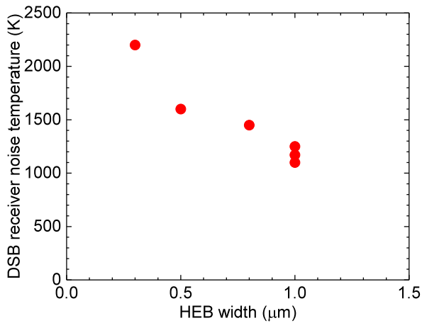
Fig. 6.19: MgB 2 HEB DSB receiver noise temperature versus HEB width.
