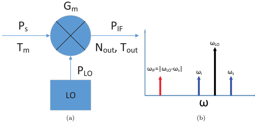
Fig. 2.5: (a) Schematic of down-converting mixer. (b) Schematic of down-conversion in a frequency domain.
