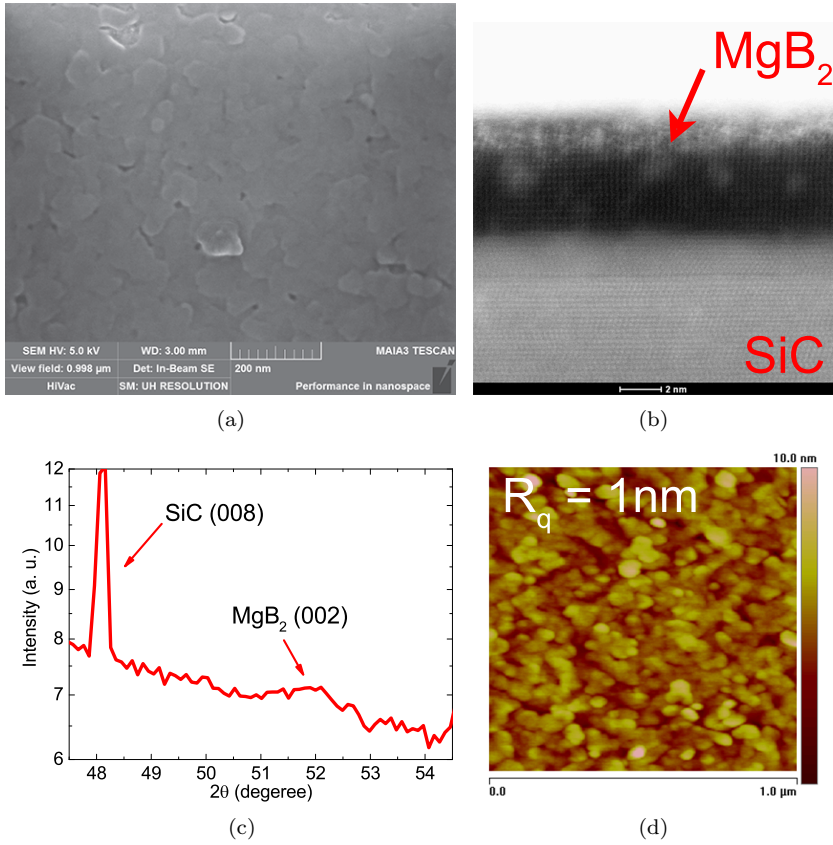
Fig. 3.8: A 5 nm thick as grown MgB_2 film. (a) SEM image. (b) TEM image. (c) XRD scan. (d) AFM image.
