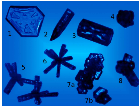
Figure 2.1: Examples of different habit classes: 1) plate, 2) bullet, 3) column (in this case, hollow column), 4) irregular, 5) rosette aggregate, 6) bullet rosette, 7) plate aggregates, and 8) column aggregate (Lindqvist et al., 2012).
