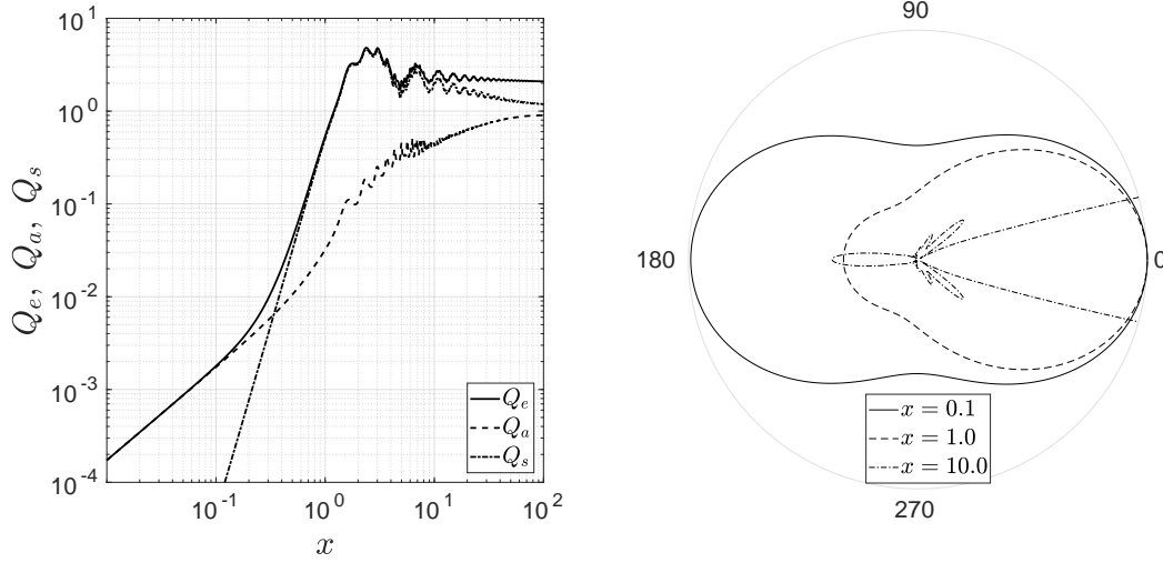
Figure 3.1: (Left) Extinction, scattering and absorption efficiency as a function of size parameter, for an ice sphere. The refractive index is n_{ice} = 1.78 + 0.011i . (Right) Angular scattering distributions ( \mathbf{Z}_{11} ) for ice spheres with three different size parameters (normalized to fit in the plot). The 0^\circ angle is defined as the direction of the incident radiation. Note that only a small portion of the pattern for x = 10 is displayed, since the forward lobe is very large in comparison to the backward lobe.
