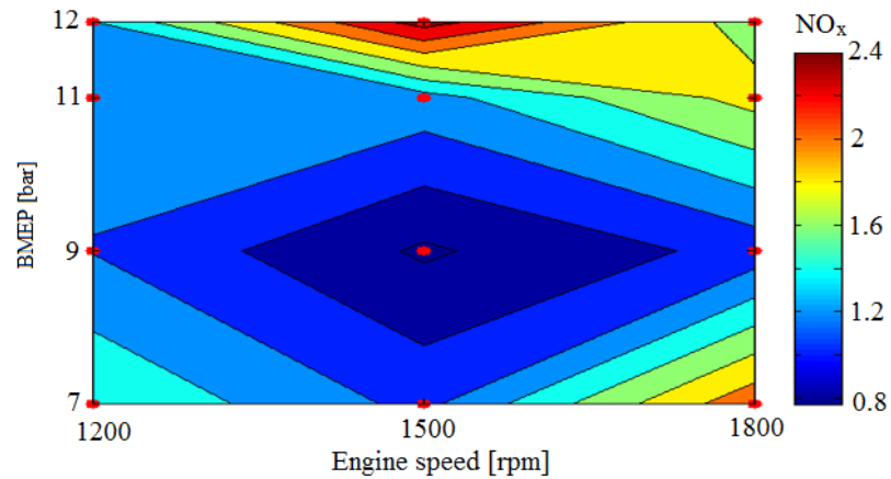
Figure 7.18: \text{NO}_x emissions for NG-Diesel RCCI at various engine speeds and loads
