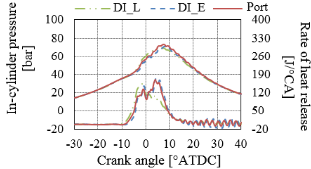
Figure 7.20: In-cylinder pressure and gross RoHR traces at PI1 SOI -48^{\circ} ATDC and PI2 SOI -15^{\circ} ATDC for three methanol injection configurations
