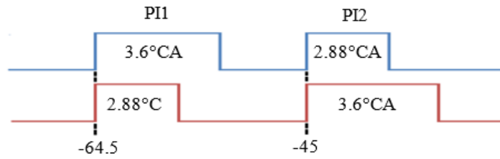
Figure 7.9: Diesel injection profiles for two test cases involving PI1 and PI2 durations of 3.6^{\circ}\text{CA}
