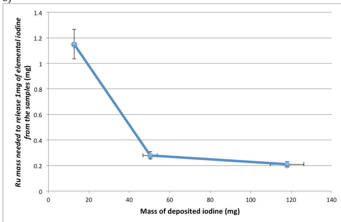
Figure 20. Dependence of Ru mass needed to release 1 mg of elemental iodine from a) aluminum, and b) zinc deposited with I_2 . Uncertainties originate from triplicates.
