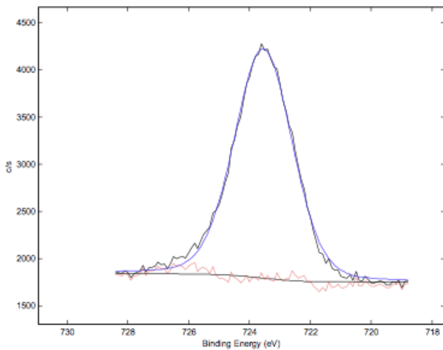
Figure B6. XPS spectrum of cesium in aerosols collected from ruthenium transport experiments with CsI injection at a temperature of 1500 K.
