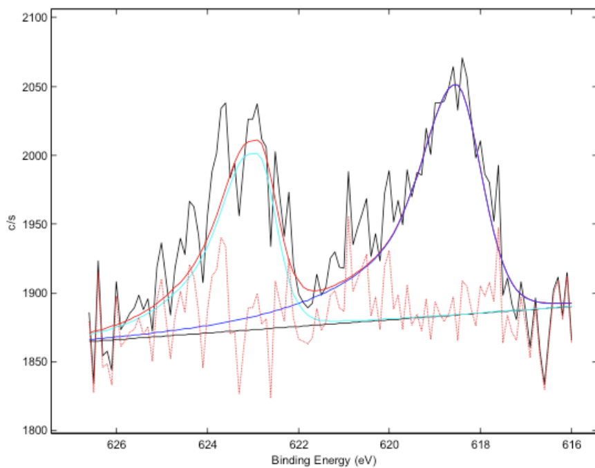
Figure B5. XPS spectrum of iodine in aerosols collected from ruthenium transport experiments with CsI injection at a temperature of 1500 K.
