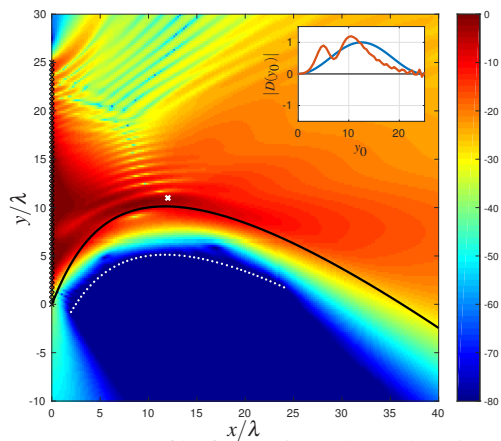
(c) Phase profile from Fig. 1(b) and optimal real weights; 52 control points were used (51 + 1)
