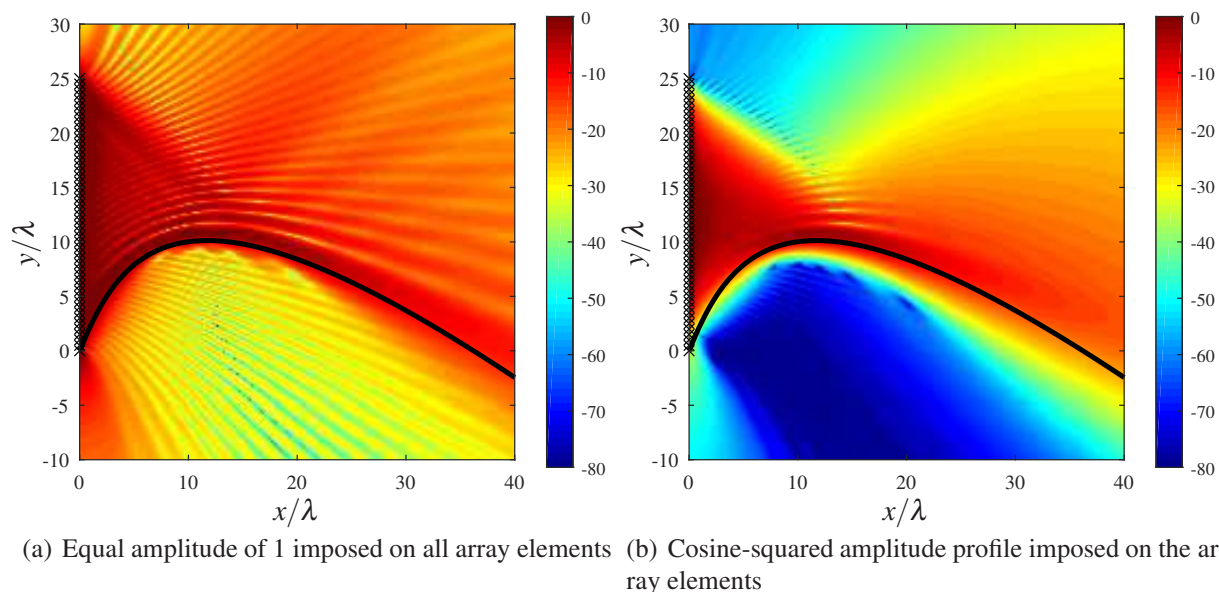
Figure 2: Magnitude in dB of the beam of a sample linear array of 51 isotropic (omnidirectional) elements of length L = 25\lambda located on the y -axis; the element spacing is \Delta y = 0.5\lambda (i.e. critically spaced); the black marks indicate the locations of the array elements; the black line represents the caustic
