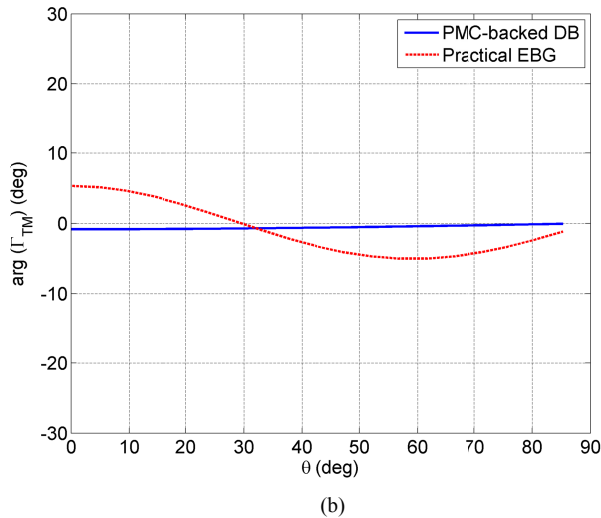
Fig. 4. Reflection coefficient phase, computed for the PMC backed uniaxial model ( h = \lambda/1000 ) and for the actual mushroom surface at 14 GHz versus the incidence angle of the impinging plane wave; (a) TE case, (b) TM case.
