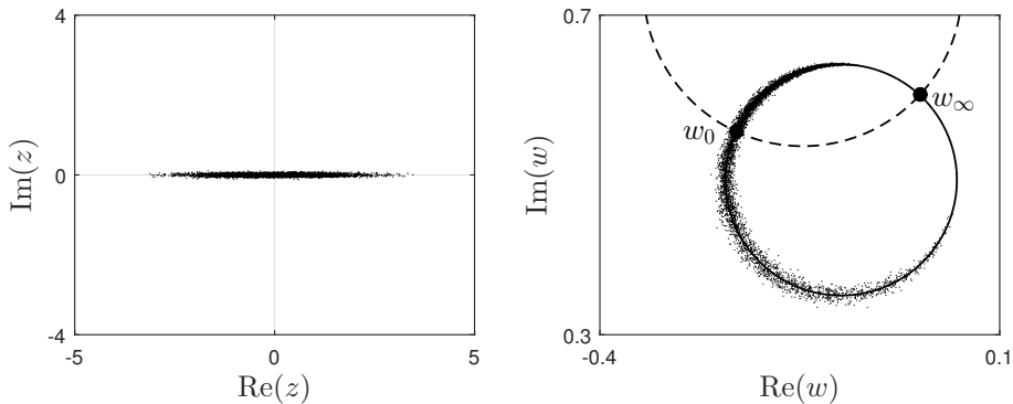
Figure 3.1: Normal distributed complex data z and its mapping through a Möbius transformation w = T(z) . Left: realisations of z in the complex plane. Right: data w in the complex plane where each point corresponds to one realisation of z . The points w_0 = T(0) and w_\infty = T(\infty) are indicated by filled circles, and the images of the real and imaginary axis under T are shown by solid and dashed curves, respectively.
