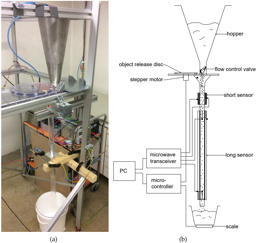
Figure 4.12: Experimental setup for studying the detection of objects in flowing granular materials. (a) photo including the short sensor, (b) schematic drawing with the short and long sensor mounted in series.
