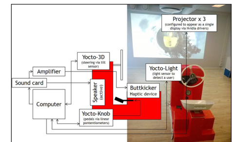
Image 1. The road grader simulator setup.
