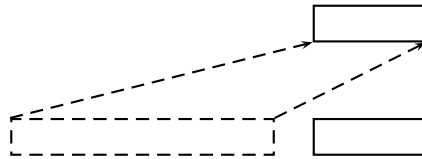
Figure 5.1: Combining the global rule with a shift function causes the preimages of two different patterns to be transferred to disjoint locations.
