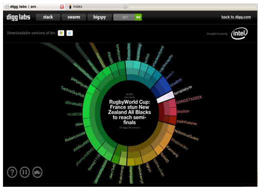
Figure 3: Digg Arc
