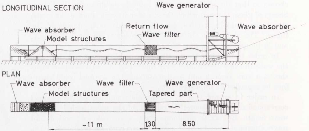
Fig. 52.1. Schematic drawing of the channel
