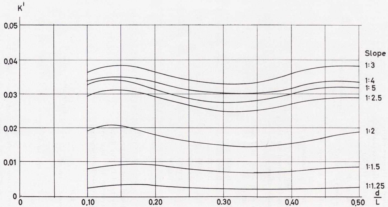
Fig. 33.1. Determination of K' (for rubble-mound structures) in terms of \frac{d}{L} and \alpha .
