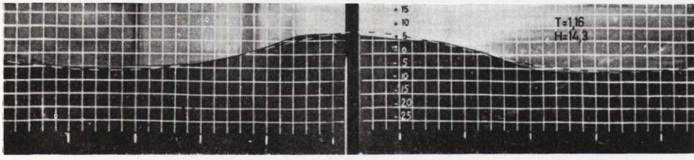
Fig. 59.1. The wave profile in the flume. Agreement between the actual wave form and the theoretical profile, dashed line
