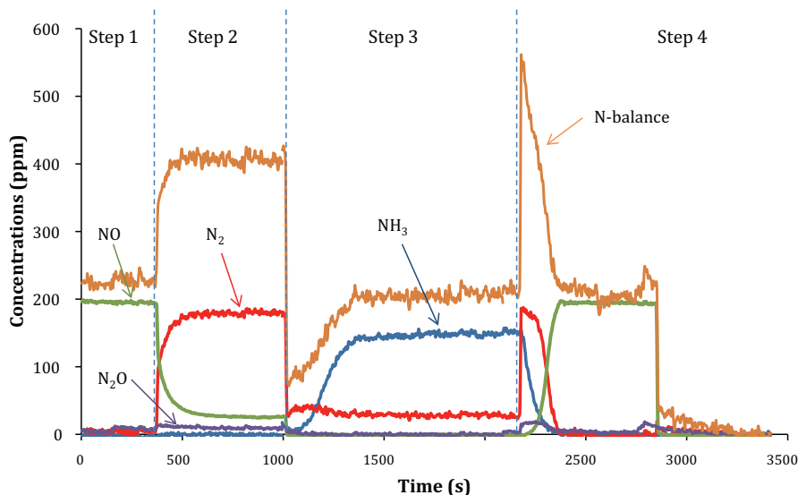
Fig. 1. Concentrations of NO, NH 3 , N 2 and N 2 O measured during the 4-step protocol at 325 °C and at the half of a Cu-BEA monolith. The nitrogen balance was calculated and also represented on the figure.
