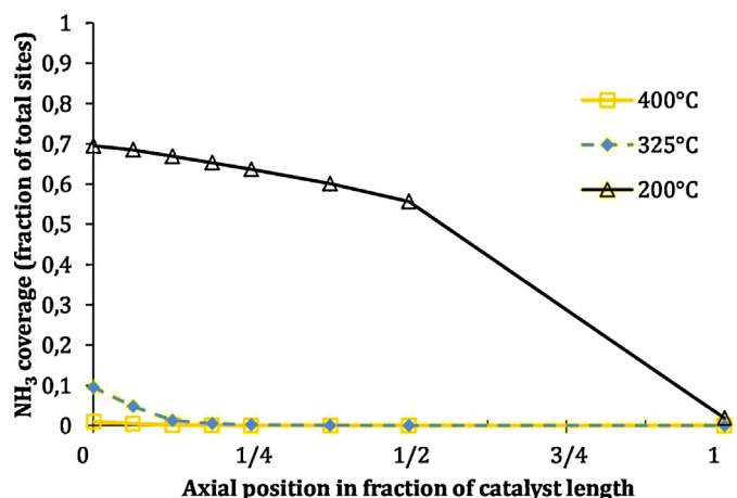
Fig. 6. Simulated NH 3 coverage and fraction of free sites during NH 3 SCR at: (a) 200 °C, (b) 325 °C and (c) 400 °C. Steady-state profile throughout the catalyst.
