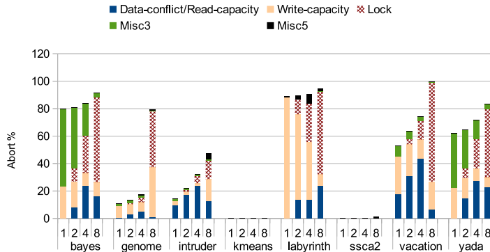
Figure 5.12: RTM Abort Distributions for STAMP Benchmarks
