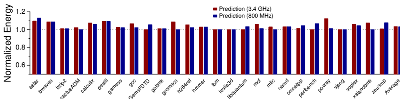
Figure 4.17: Energy Expenditure at P(3.4)_E and P(0.8)_E Normalized to F_E for SPEC 2006 Benchmarks
