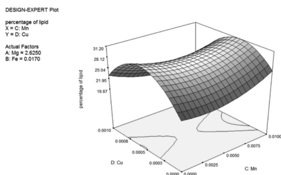
FIGURE 6. Pattern of interaction between Mn^{2+} and Cu^{2+}
