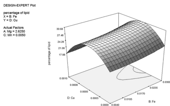
FIGURE 5. Pattern of interaction between Fe^{3+} and Cu^{2+}
