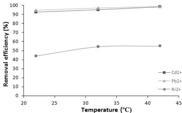
Fig. 1. Temperature effect on the adsorption of Pb 2+ , Cd 2+ and Ni 2+ onto CScPA
