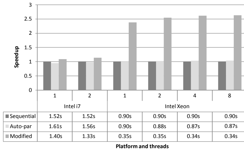
Fig. 9: Speedup and executing time of the edge-detection kernel on the (a) Intel i7 platform and (b) Intel Xeon platform. In the modified version using the feedback suggestions, all loops were parallelized. In the unmodified the outer loop were not parallelized.
