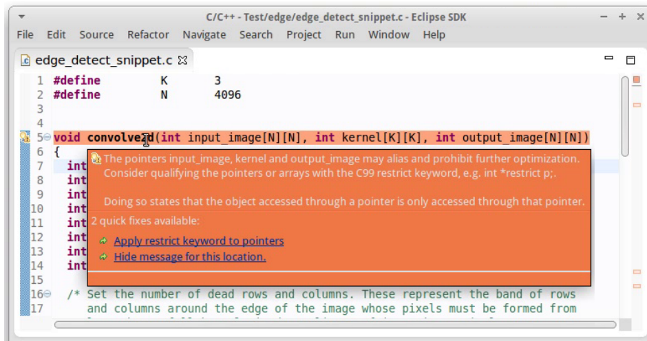
Fig. 8: Marker suggesting adding the restrict keyword to the three array arguments.
