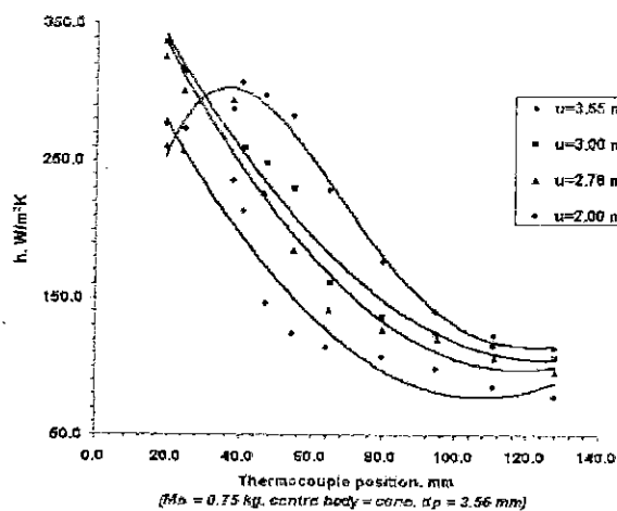
Fig. 7. h vs U at different heights above distributor.
