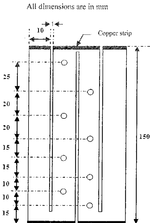
Fig. 3. Constantan heater foil and thermocouple location.
