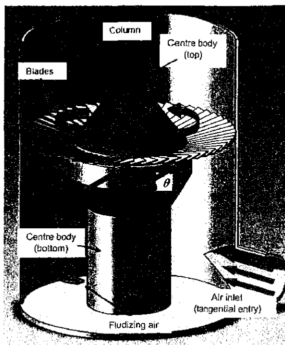
Fig. 1. Basic configuration of a swirling fluidized bed.
