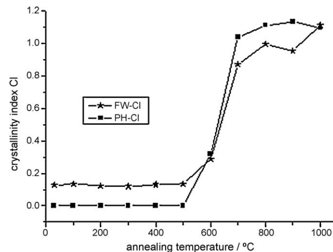
Fig. 2. Crystallinity indices as a function of annealing temperature.
