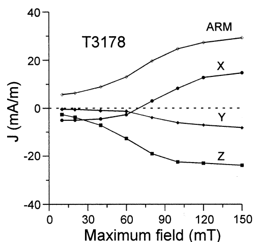
Figure 13. Intensity and single components of ARM during AF demagnetization (ARM acquired in a DC field of 50 \mu\text{T} along -z -axis, see text).
