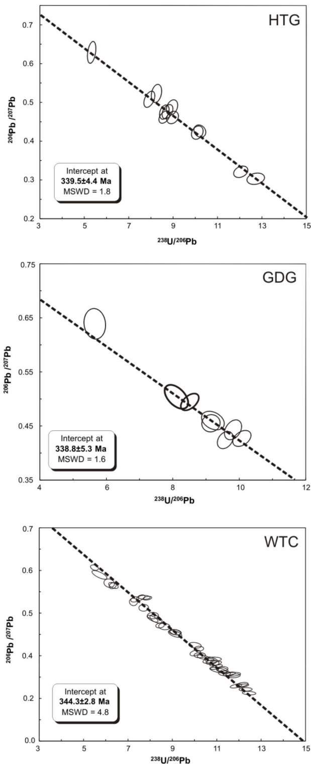
Fig. 5. Tera-Wasserburg concordia diagrams anchored through common Pb for HTG (a), GDG (b) and WTC (c).
