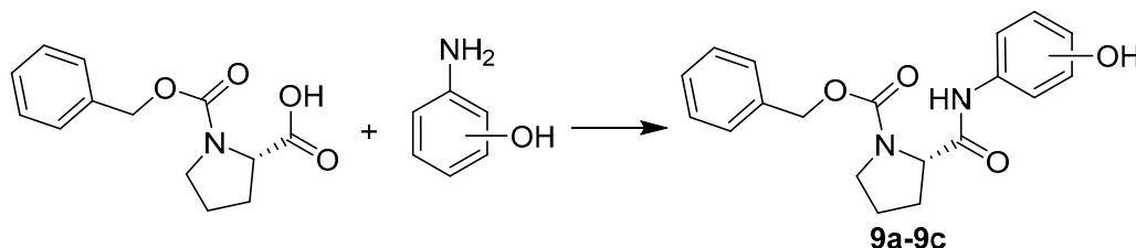
Scheme 2. Synthesis of benzyl (2 S )-2-[(hydroxyphenyl)carbamoyl]pyrrolidine-1-carboxylates 9a–9c . Reagents and conditions: triethylamine, tetrahydrofuran, ethyl chloroformate, room temperature, argon atmosphere.
