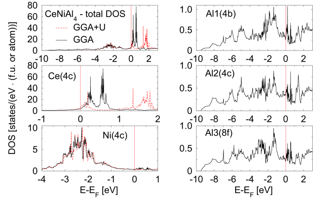
Fig. 2. Total and local DOS plots for CeNiAl 4 : calculations performed for GGA and GGA+U, where U for Ce 4 f electrons is equal to 6 eV and for Ni 3 d ones is equal to 3 eV.
