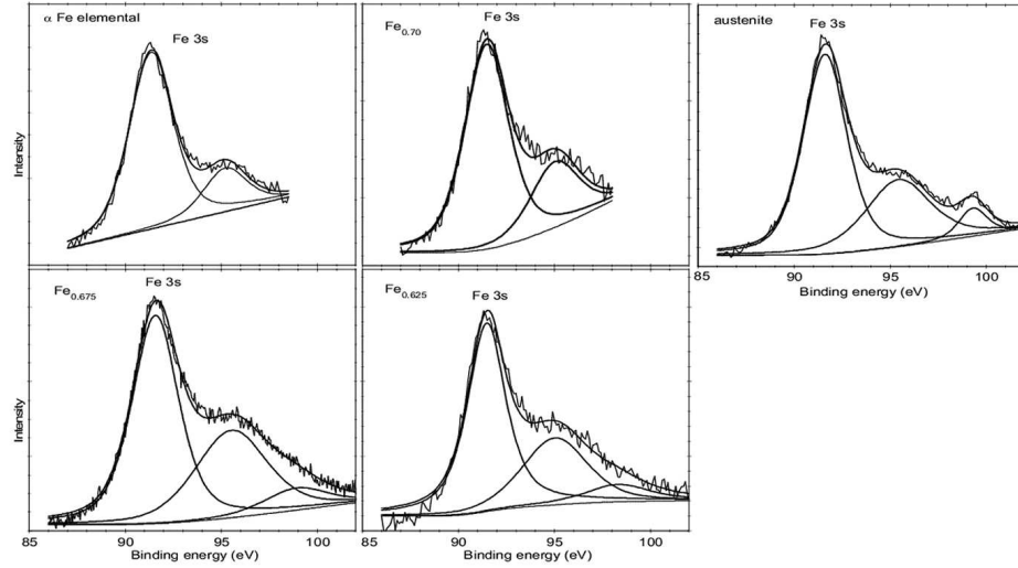
Fig. 4. The Fe 3s spectra of the pure Fe, austenitic steel and \text{Fe}_{1-x}\text{Ni}_x ( x = 0.30, 0.325, 0.375 ) alloys, after subtraction of background.
