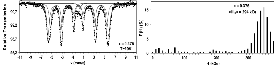
Fig. 2. The Mössbauer spectra and respective hyperfine field (HF) distribution for \text{Fe}_{0.625}\text{Ni}_{0.375} at temperature \approx 20 K.
