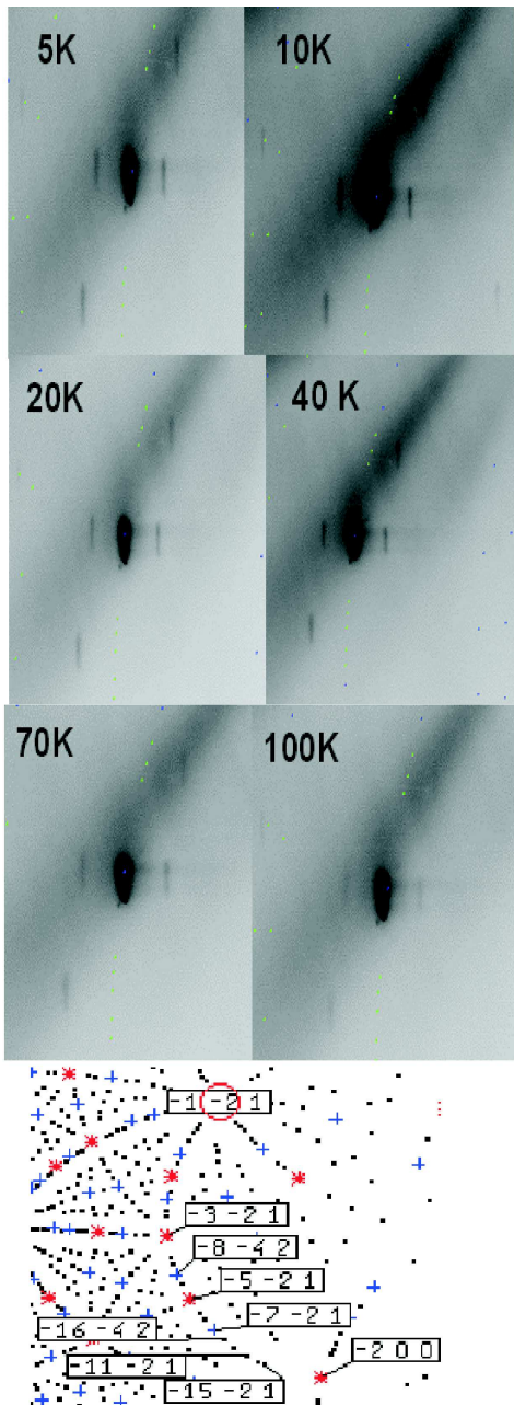
Fig. 3. Main nuclear spot ( \bar{2}00 ) to which four magnetic satellites: (\pm\varepsilon, \pm\varepsilon, 0) vanishing above 100 K are attached. Similarly, not-allowed but well-visible magnetic satellites of (\bar{1}k1) nuclear reflections were observed.
