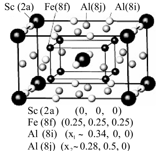
Fig. 1. Crystal structure of \text{ScFe}_4\text{Al}_8 consisting 26 atoms (two molecules) per unit cell I4/mmm with the a = 8.623(5) \text{ \AA} and c = 5.008(4) \text{ \AA} cell parameters at 8(2) K [1].
