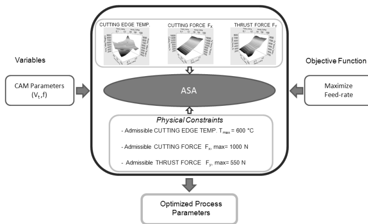
Figure 5: Scheme of optimization problem definition.
