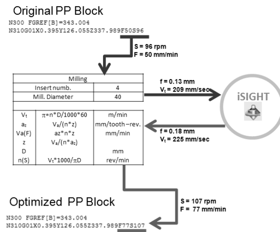
Figure 6: Flowchart of input-output process parameters optimization.
