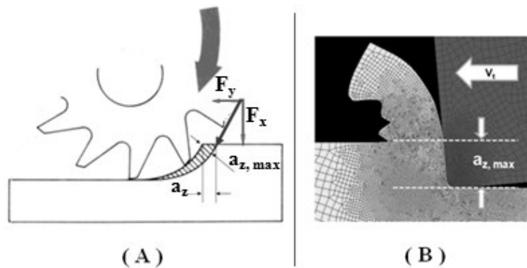
Figure 2: (A) Climb mill operation ; (B) FE simplified 2D model.
