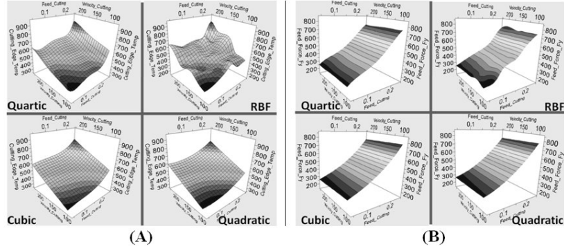
Figure 3: Metamodels shapes comparison for the four adopted techniques. (A) for T_{max} response; (B) for F_y response.
