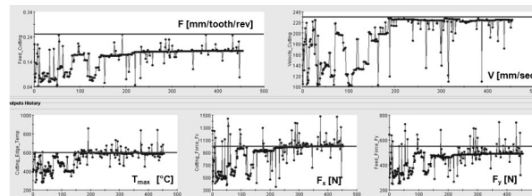
Figure 7: ASA iterations history.
