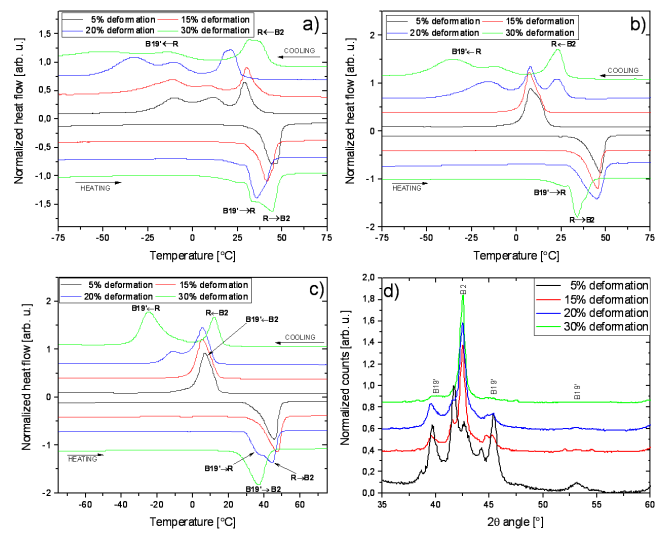
Fig. 3. DSC curves for sample annealed at (a) 400^\circ\text{C} , (b) 450^\circ\text{C} , (c) 500^\circ\text{C} for 15 min, (d) XRD pattern for sample annealed at 450^\circ\text{C} for 15 min.
