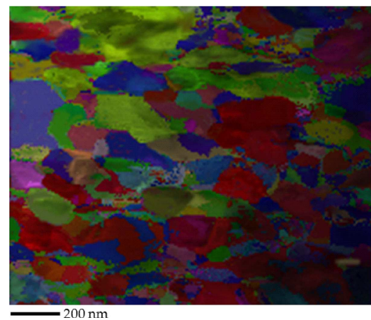
Fig. 8. Orientation map of 30% cold rolled material annealed at 500 °C obtained using PED method.
