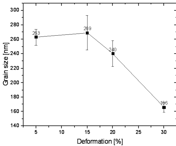
Fig. 5. Average grain size of 5%, 15%, 20% and 30% cold rolled material annealed at 500 °C for 15 min.
