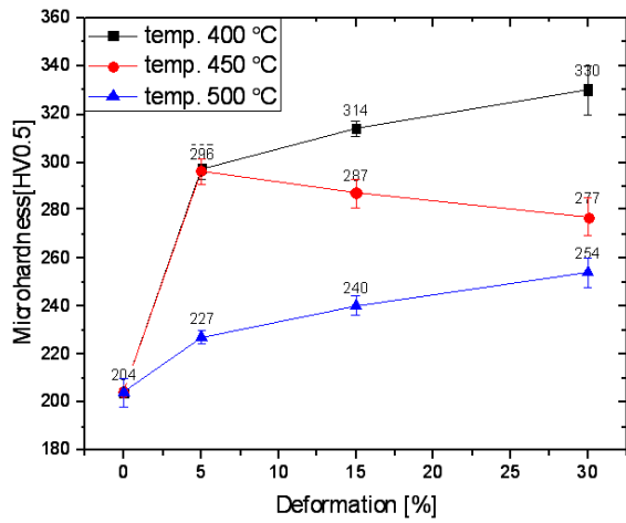
Fig. 4. Microhardness for sample annealed at 400 °C, 450 °C and 500 °C for 15 min.
