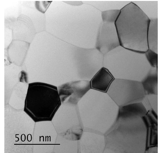
Fig. 7. TEM image of 20% cold rolled material annealed at 500 °C — fine grains of parental phase.
