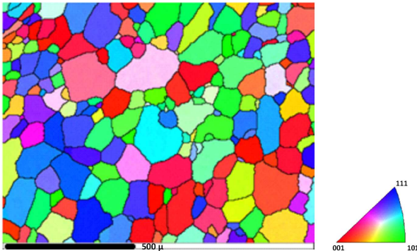
Fig. 2. Orientation map recorded for material without thermo-mechanical treatment obtained by EBSD measurements.
