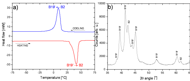
Fig. 1. (a) DSC curves and (b) XRD diffraction pattern for material without thermo-mechanical treatment.
