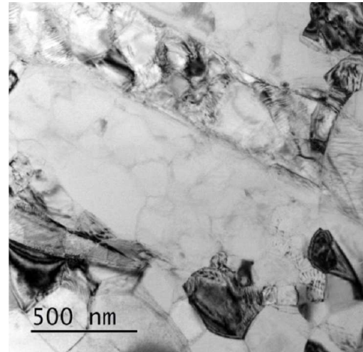
Fig. 6. TEM image of 5% cold rolled material annealed at 400 °C.
