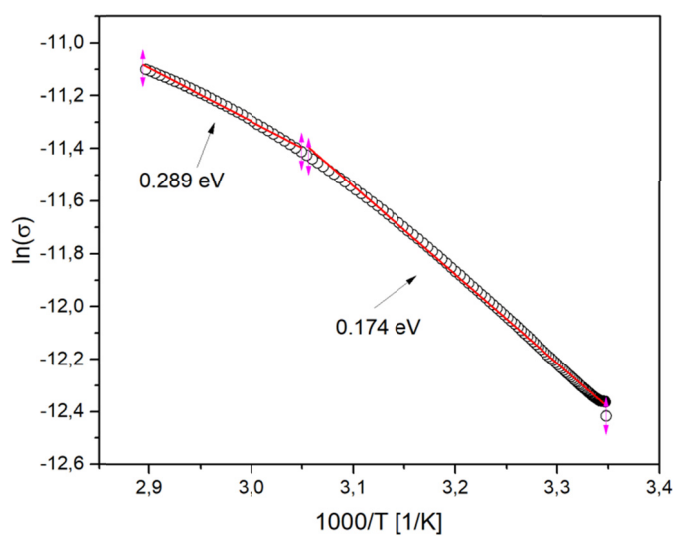
Fig. 5. The dependence of the \ln(\nu(1000/T)) for \text{Bi}_{0.9}\text{Dy}_{0.1}\text{FeO}_3
