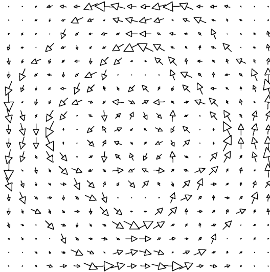
Fig. 1. Current distribution originating from external magnetic field calculated for a 20 \times 20 cluster with fixed boundary conditions. ea^2H_z/(\hbar c) = 0.1 was used.
