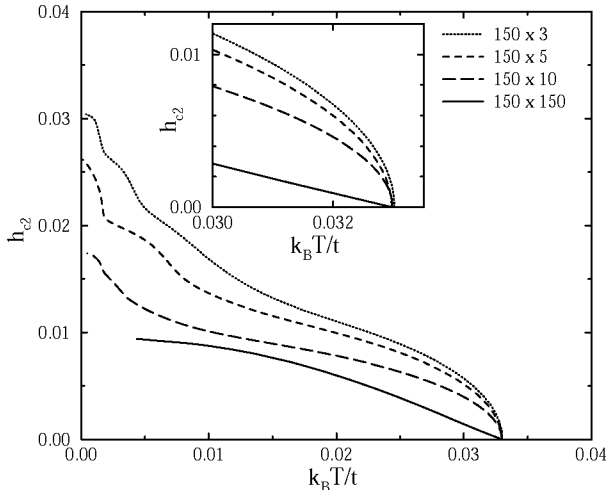
Fig. 3. Comparison of the upper critical field for a homogeneous system (continuous line) and systems with stripes of different width (3, 5 and 10 lattice sites).
