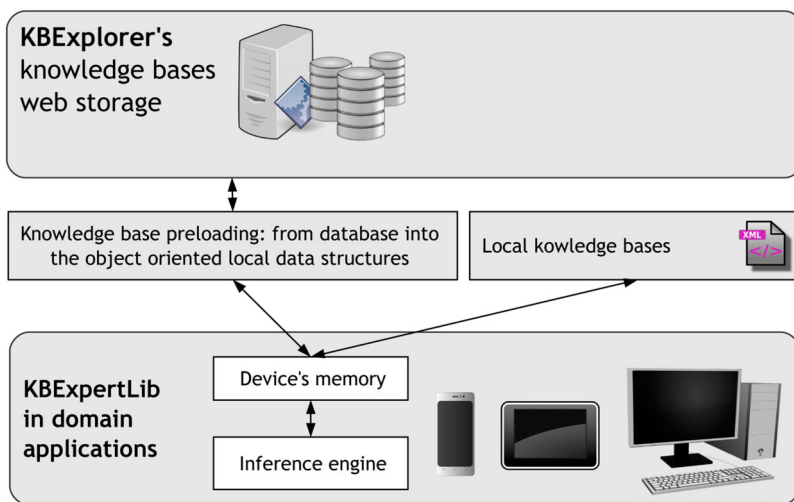
Figure 2. First approach: inference as a local process.
