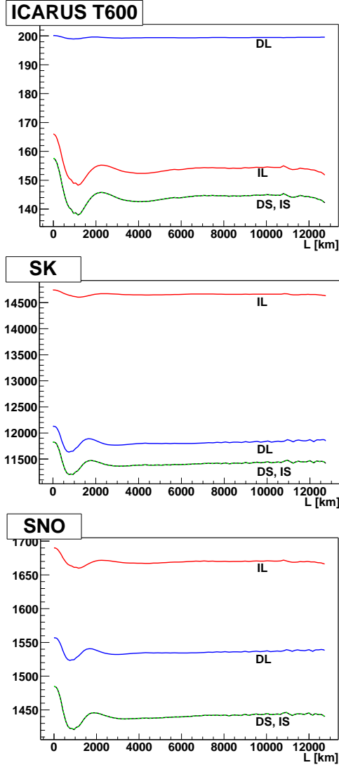
Fig. 2. The expected number of supernova neutrino interactions in ICARUS T600 (600 tons of liquid argon), SK (32 kttons of light water) and SNO (1 kton of heavy water, 1.7 kttons of light water) detectors as a function of the distance, L , neutrinos traveled in the Earth, for different combinations of mass hierarchy and \theta_{13} (DL — Direct mass hierarchy and Large \theta_{13} , IL — Inverted mass hierarchy and Large \theta_{13} , DS — Direct mass hierarchy and Small \theta_{13} , IS — Inverted mass hierarchy and Small \theta_{13} ). For details see the description in the text.
