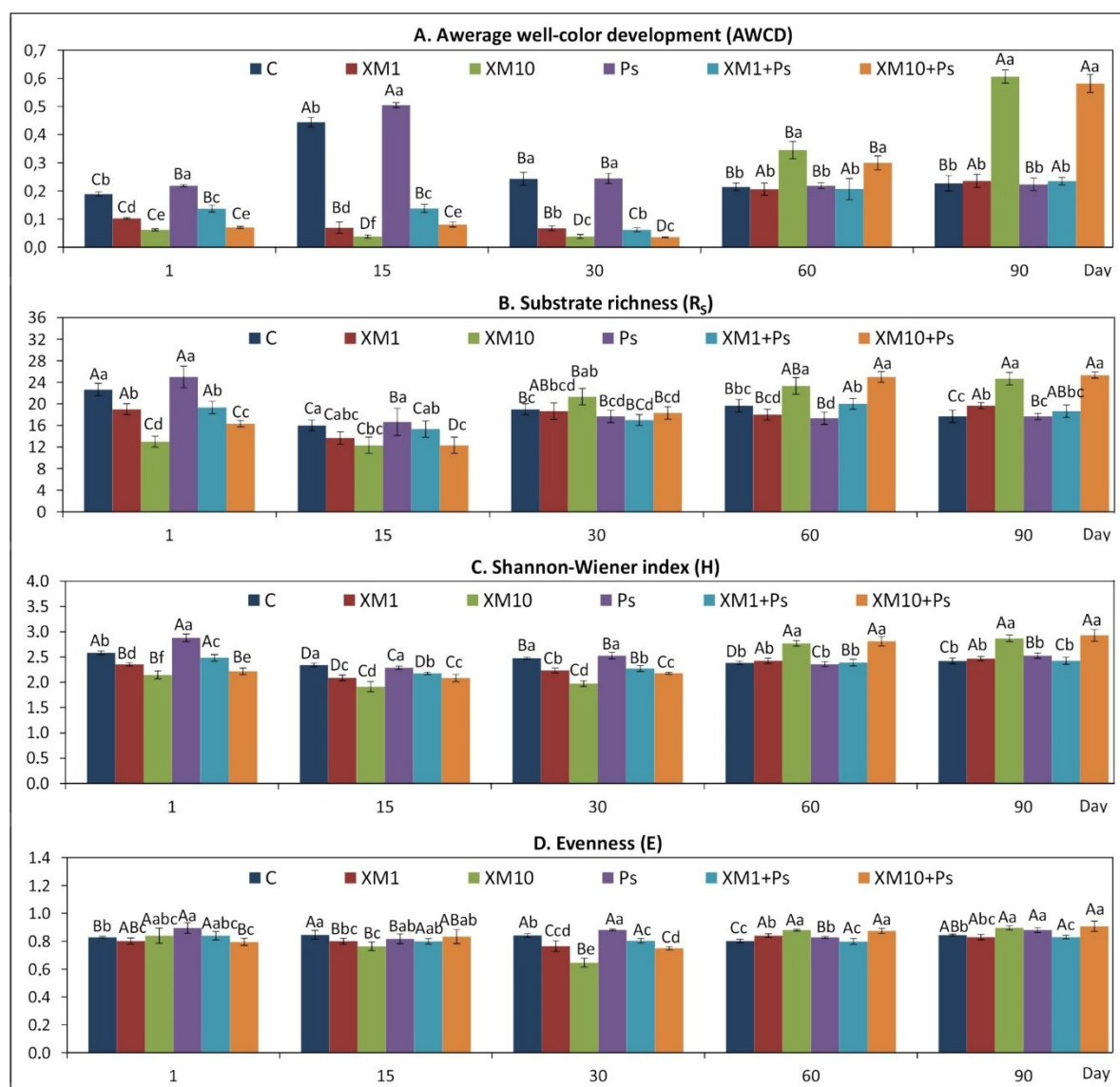
Figure 2. Effect of XM and/or strain MC1 on the values of the CLPP indices, i.e., AWCD (A), Rs (B), H (C) and E (D). The data presented are the means of three replicates with standard deviations. Significant differences (LSD test, p < 0.05 ) between treatments at the same sampling time and between sampling times within the same treatments are denoted with different lower and uppercase letters, respectively. The treatment abbreviations are explained in Figure 1.
