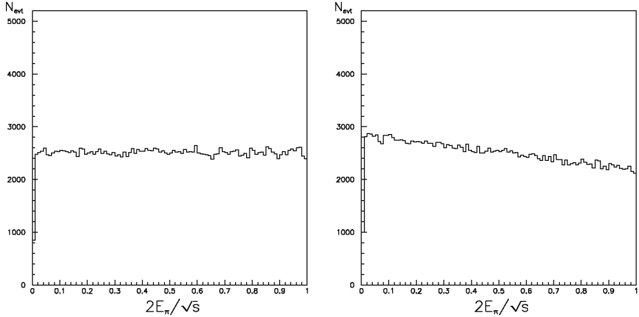
Fig. 2. Single \pi energy spectrum in the case of \tau produced from H (left-hand side) or Z (right-hand side). \sqrt{s} = m_H or \sqrt{s} = m_Z respectively. Energies are calculated in the rest frame of Higgs boson (or Z ).
