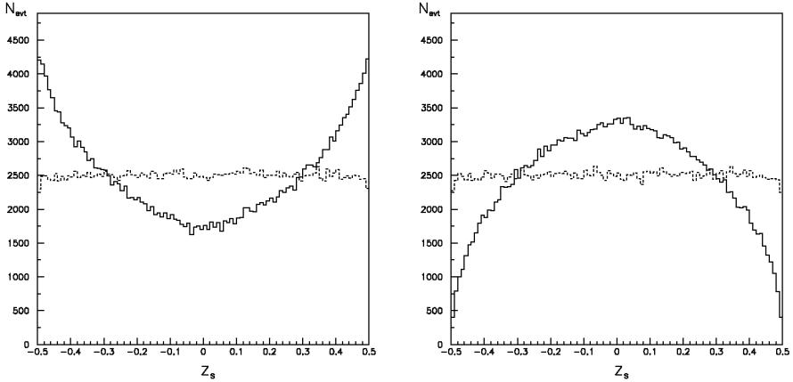
Fig. 4. Expected number of events as the function of z_s variable. Left-hand side plot for H , right-hand side for Z . Continuous line with spin effects included, dotted line with spin effects switched off.
