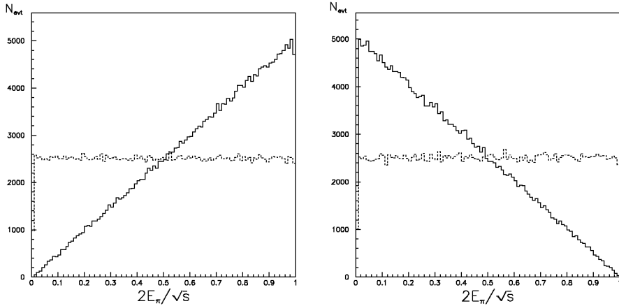
Fig. 3. Single \pi energy spectrum in the case of \tau produced from H^\pm (left-hand side) or W^\pm (right-hand side). \sqrt{s} = m_{H^\pm} or \sqrt{s} = m_{W^\pm} , respectively. Energies are calculated in the rest frame of H^\pm (or W^\pm ). Continuous line with spin effects included, dotted line with spin effects switched off.
