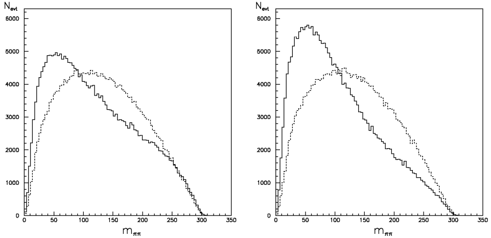
Fig. 7. The \pi^+\pi^- invariant mass distribution for u\bar{u} \rightarrow Z/\gamma^* (left-hand plot) and d\bar{d} \rightarrow Z/\gamma^* (right-hand plot) produced with cms energy of 300 GeV. Continuous line with spin effects included, dotted line with spin effects switched off.
