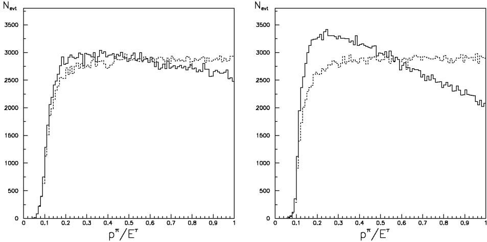
Fig. 8. The \pi energy spectrum in the laboratory frame, after basic selection as specified in text, for Higgs boson (left-hand side) and Z/\gamma^* (right-hand side). Continuous line with spin effects included, dotted line with spin effects switched off.
