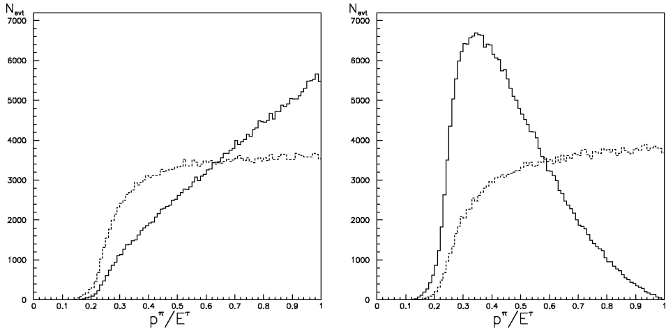
Fig. 11. Distribution of p^\pi/E^\tau after basic selection and in the laboratory frame. On the left plot for H^\pm ( m_H = 130 GeV), on the right for W^\pm . Continuous line with spin effects included, dotted line with spin effects switched off.
