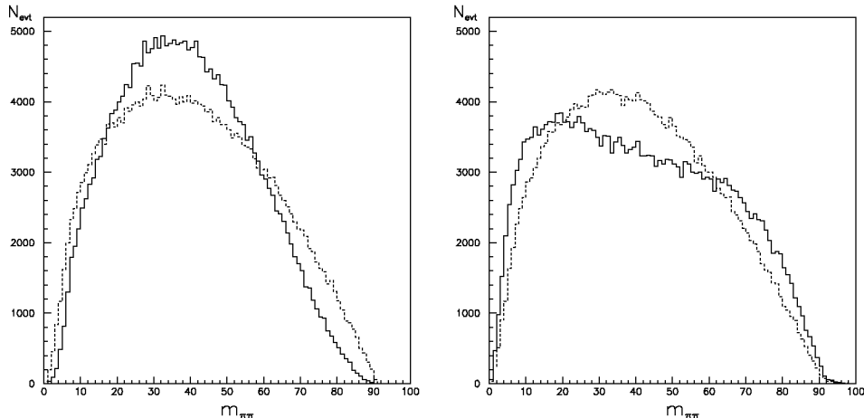
Fig. 6. The \pi^+\pi^- invariant mass distribution. Left-hand side plot for H ; right-hand side for Z/\gamma^* . Continuous line with spin effects included, dotted line with spin effects switched off. In the two cases respectively \sqrt{s} = m_H = m_Z .
