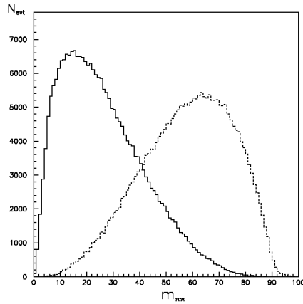
Fig. 5. The \pi^+\pi^- invariant mass distribution for \sqrt{s} = m_Z . Continuous line for pure (-, -) dotted line for pure (+, +) spin configurations.
