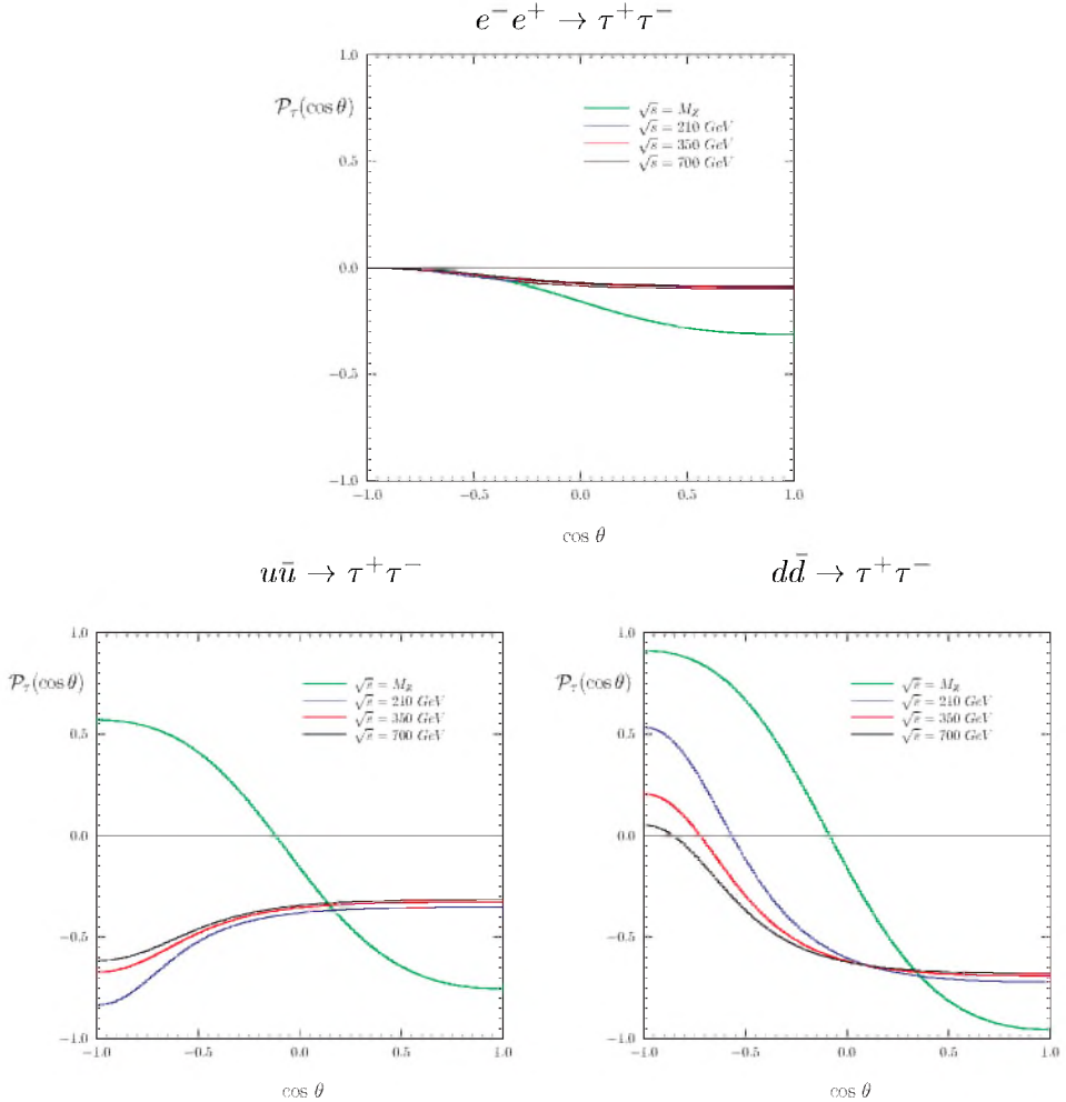
Fig. 1. Tests of the TAUOLA universal interface. The \tau lepton polarisation as a function of \cos\theta . We have used \sqrt{s} = M_Z, 210, 350 and 700 GeV.
