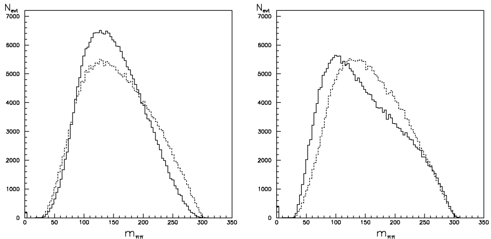
Fig. 10. The \pi^+\pi^- invariant mass distribution after basic selection. On the left for Higgs boson, on the right for Z/\gamma^* . Continuous line with spin effects included, dotted line with spin effects switched off. The Higgs boson mass was assumed to be 300 GeV (see text).
