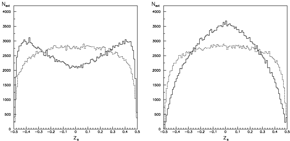
Fig. 9. The expected number of events as a function of the \pi^+\pi^- energy–energy correlation variable z_s , basic selection as specified in the text. Distributions are shown for Higgs boson (left-hand side) and Z^*/\gamma^* (right-hand side). Continuous line with spin effects included, dotted line with spin effects switched off.
