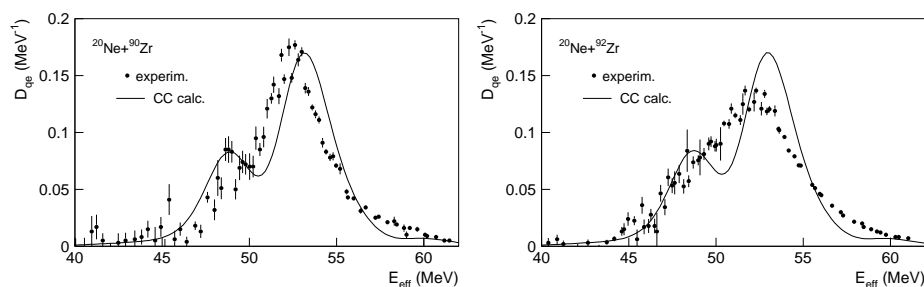
Fig. 1. Barrier height distributions for ^{20}\text{Ne}+^{90}\text{Zr} (left panel) and ^{20}\text{Ne}+^{92}\text{Zr} (right panel) compared with the results of coupled channels calculations (Ref. [4]).
