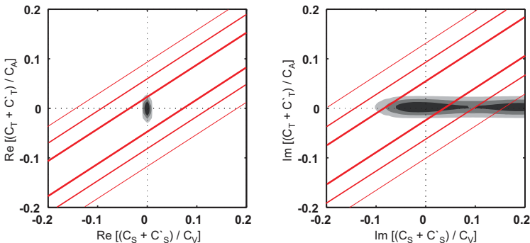
Fig. 2. Experimental bounds on the scalar vs. tensor normalized couplings. Lines represent the result of this work 1, 2 and 3 \sigma respectively, while the grey areas illustrate corresponding limitations from former existing experiments as collected in [13].
