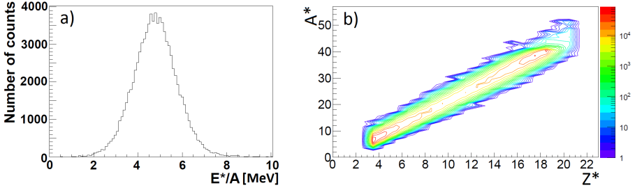
Fig. 4. Distribution of (a) the excitation energy per nucleon of the intermediate mass fragments, (b) mass versus charge of selected primary fragments, generated by the QMD model for the reaction time: t = 300 \text{ fm}/c .
