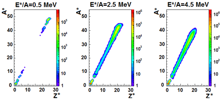
Fig. 5. De-excitation of the primary nucleus Z^* = 25 , A^* = 49 for different excitation energy per nucleon in the range of 0.5–4.5 MeV.
