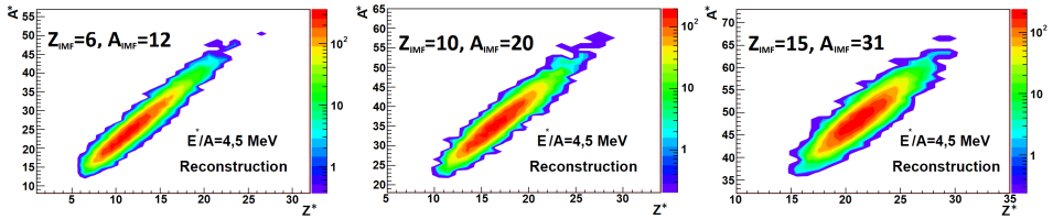
Fig. 7. Group of particles reconstructed from a particular secondary nucleus.
