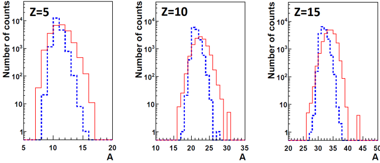
Fig. 2. Isotopic distribution from the QMD (solid line) and GEMINI (dotted line) models.
