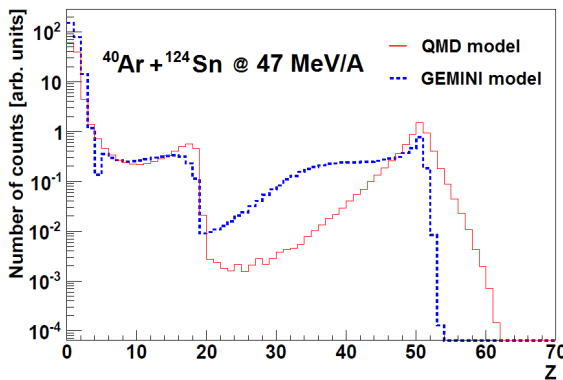
Fig.1. Comparison between primary (QMD model — solid line) and secondary (GEMINI — dotted line) fragments of heavy ion reaction for ^{40}\text{Ar} + ^{124}\text{Sn} at 47 \text{ MeV}/A .
