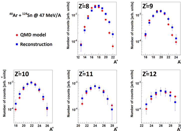
Fig. 8. Comparison of isotopic distribution of the primary fragments obtained from the reconstruction procedure (squares) and QMD model (dots). The vertical bars correspond to the statistical errors.
