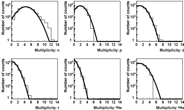
Fig. 6. The Gaussian fit of the light particles (LP): n, p, d, t, {}^3\text{He}, {}^4\text{He} corresponding with second decays of nucleus: Z = 10, A = 20, E^*/A = 4.5 MeV.
