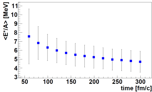
Fig. 3. Time dependence of average excitation energy per nucleon for intermediate mass fragments. Statistical errors are defined as the standard deviation from a particular distributions.
