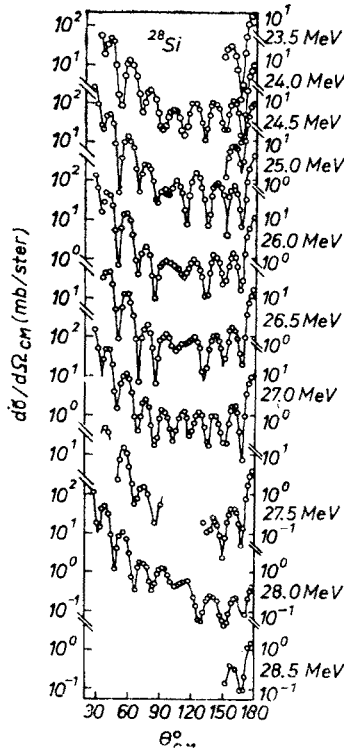
Fig. 1. Angular distributions of elastically scattered alpha particles from ^{28}\text{Si} in the energy range from 23.5 to 28.5 MeV
