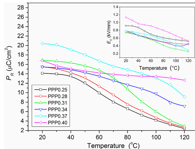
Figure 10. The temperature dependencies of remnant polarization P_R and coercive field E_C (inside) for PMN–PT–PS solid solutions.
