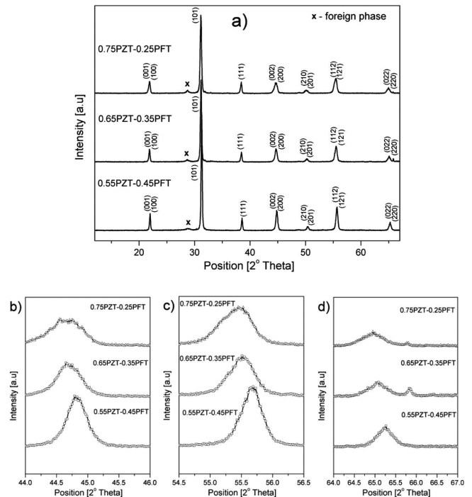
Fig. 2. XRD patterns for synthesized PZT-PFT type powders
