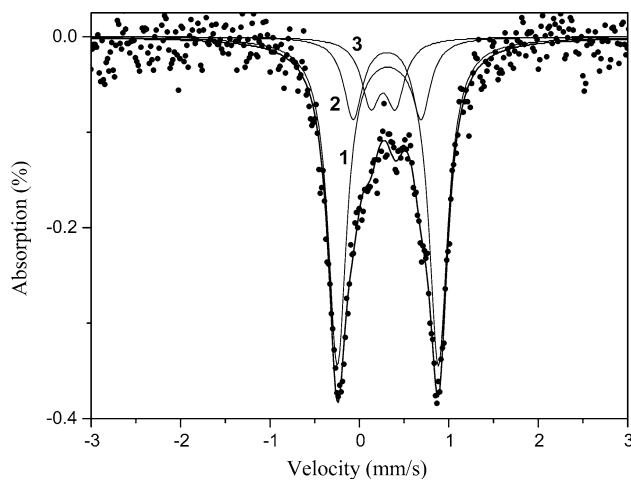
Figure 2 ^{57}\text{Fe} Mössbauer spectrum of \text{Bi}_{12}\text{MnO}_{20} – \text{BiMn}_2\text{O}_5 –Fe ceramics, obtained at room temperature. The fitted sub-spectra are presented in the spectrum.
